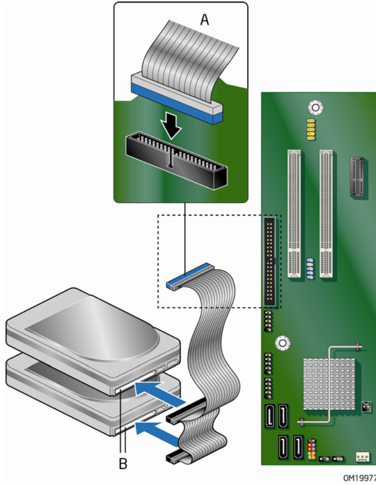
Figure 21. Connecting the IDE Cable
