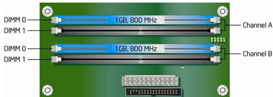
Figure 13. Dual Channel Memory Configuration with Two DIMMs
