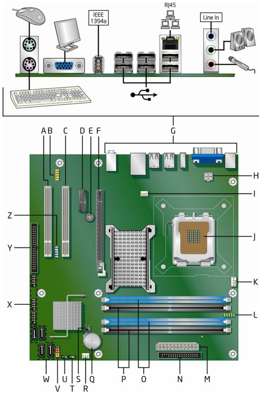
Figure 1. Desktop Board DG33BU Components
