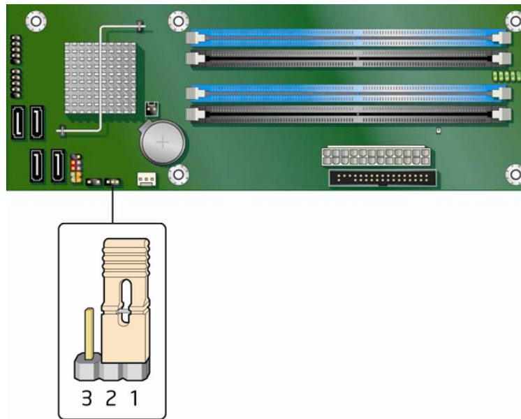
Figure 27. Location of the BIOS Configuration Jumper Block
