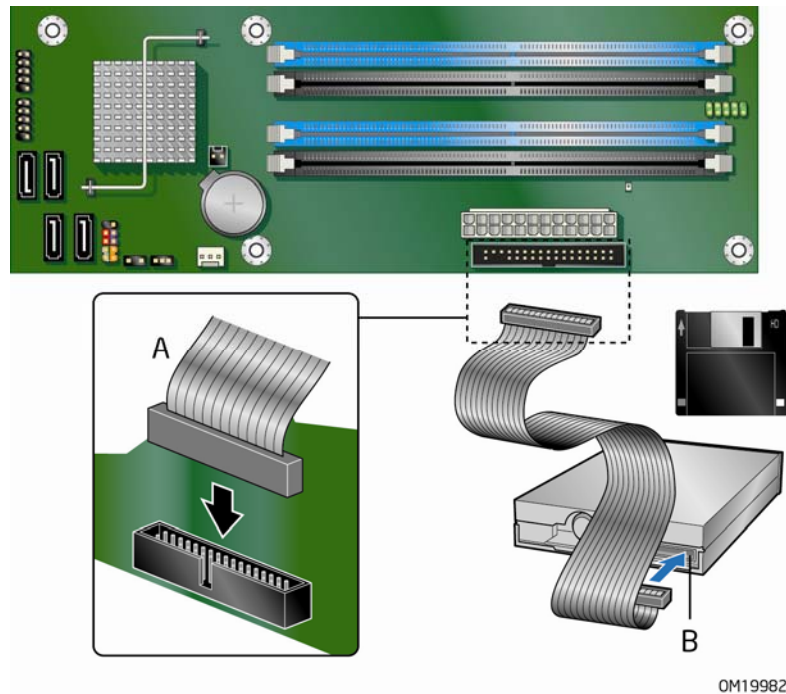
Figure 20. Connecting the Diskette Drive Cable
