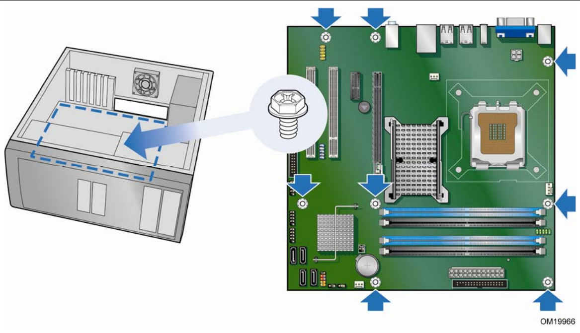
Figure 5. Desktop Board DG33BU Mounting Screw Hole Locations
