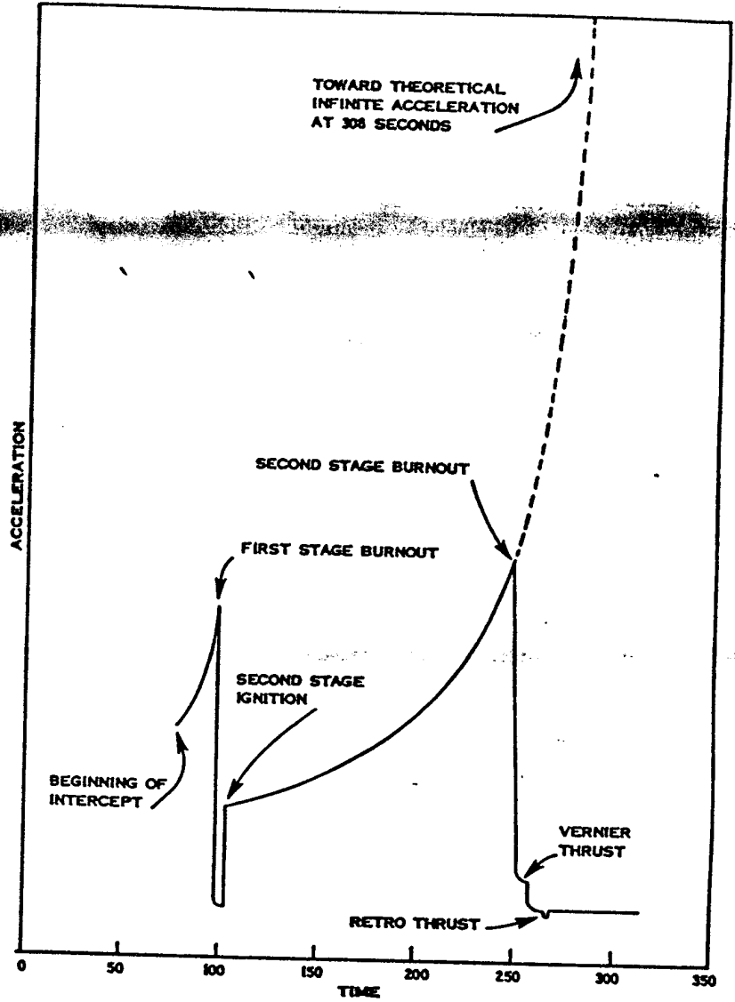
FIGURE 2. Typical Missile Acceleration History.
