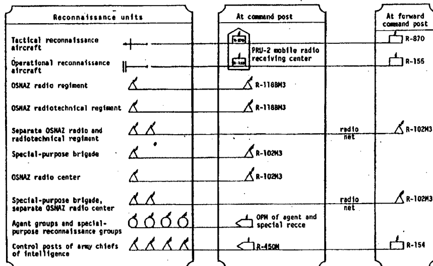
Diagram 3. Basic diagram of the organization of communications of the control post of the chief of intelligence with reconnaissance organs and units
