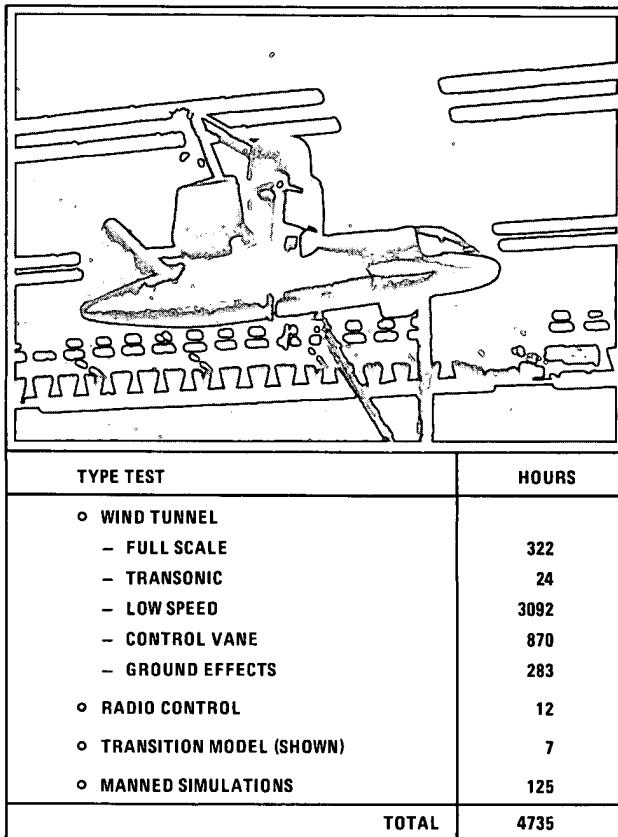
Figure 27 Design 698 Testing
