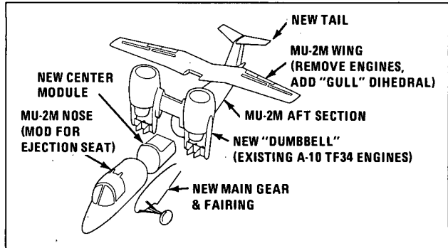
Figure 33 Demonstrator Fabrication Approach
