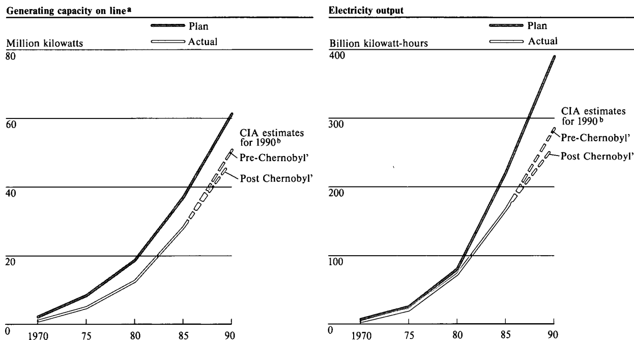
Figure 4 Soviet Nuclear Power: Performance Versus Plan
