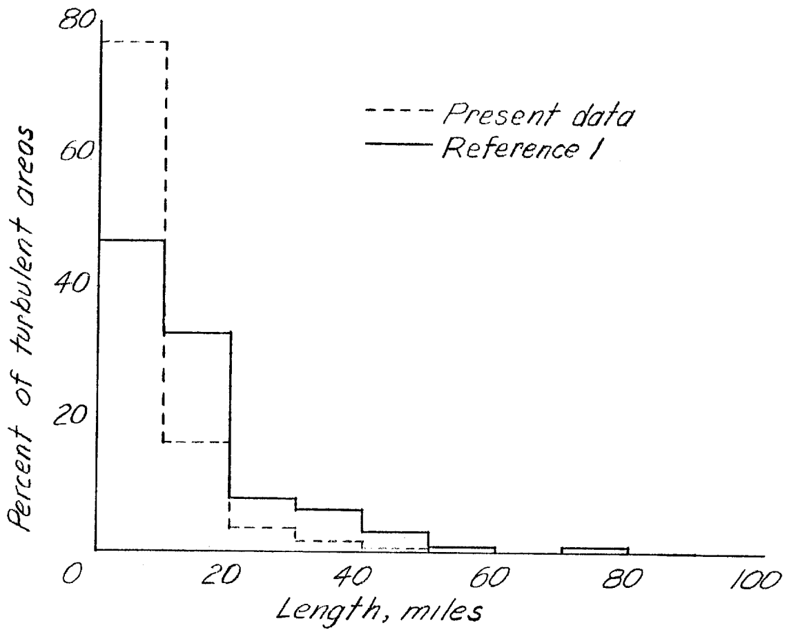
Figure 5.- Distribution of the lengths of turbulent areas for altitudes between 20,000 and 55,000 feet.
