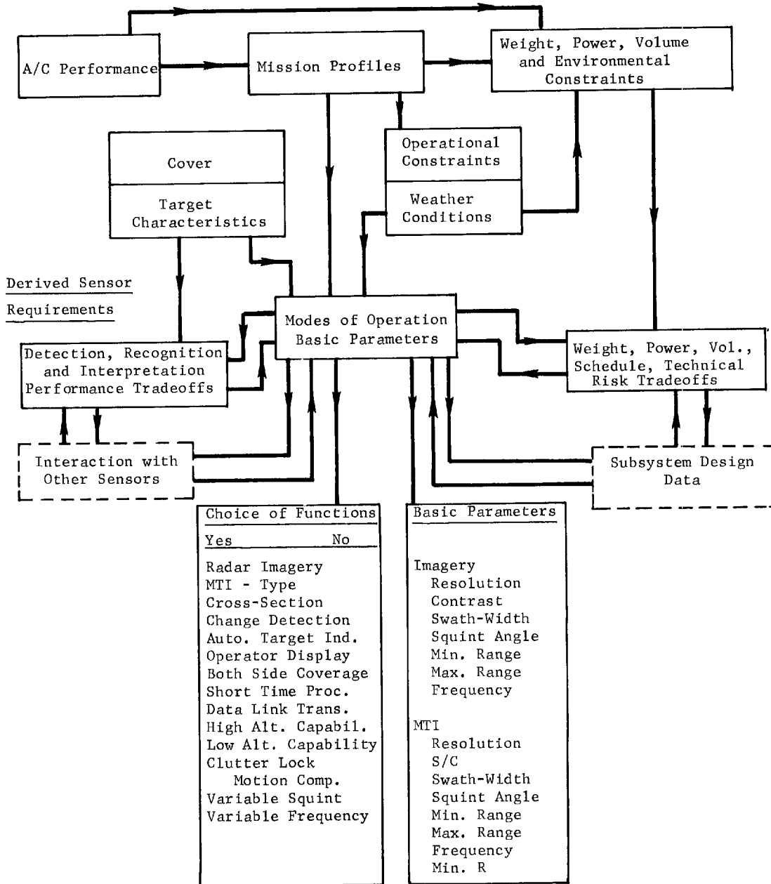
Fig. 4-24 — Interconnection between requirements and system parameters for a synthetic array radar.
