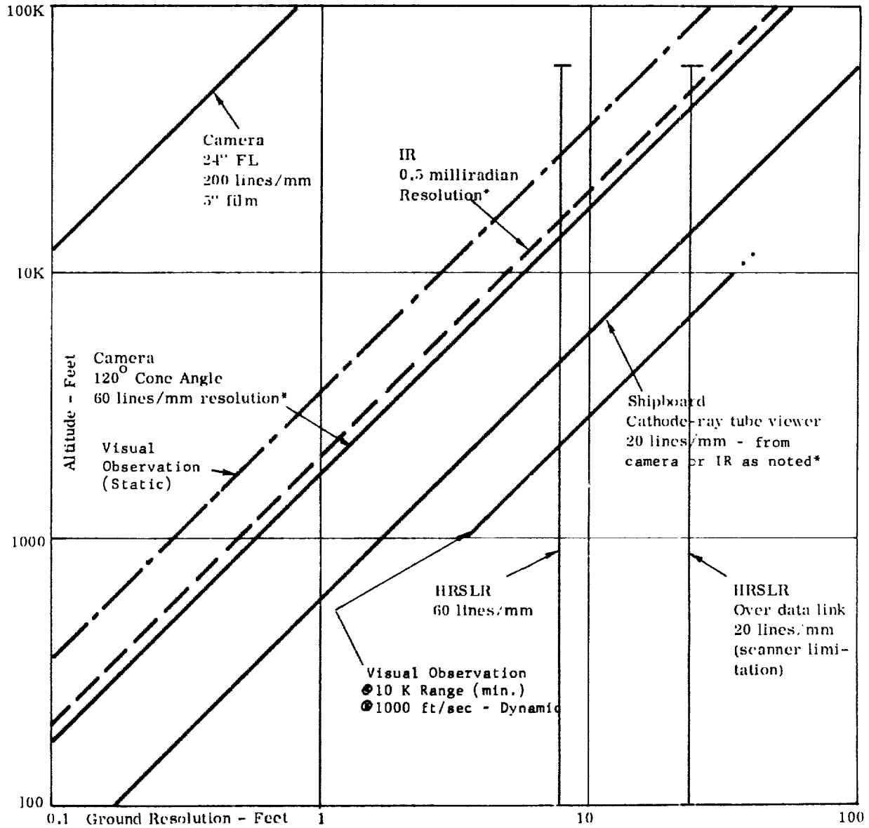
Fig. 2-3 — Imaging sensor
