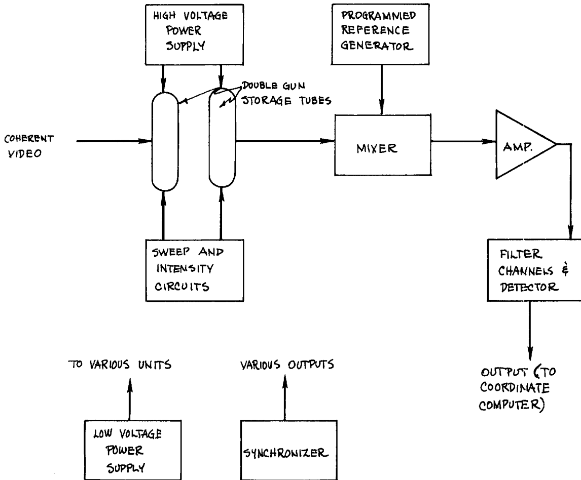
Fig. 4-32 — Real time storage tube MTI processor.
