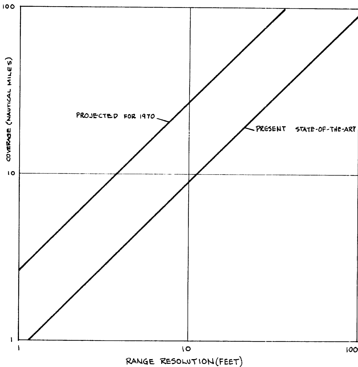
Fig. 4-31 — Total range swath per 100 pounds of recorder.
