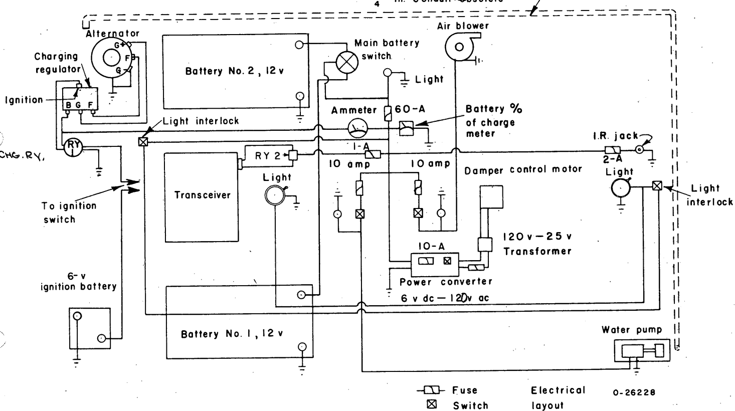
FIGURE 13 B. ELECTRICAL SYSTEM PICTORIAL
