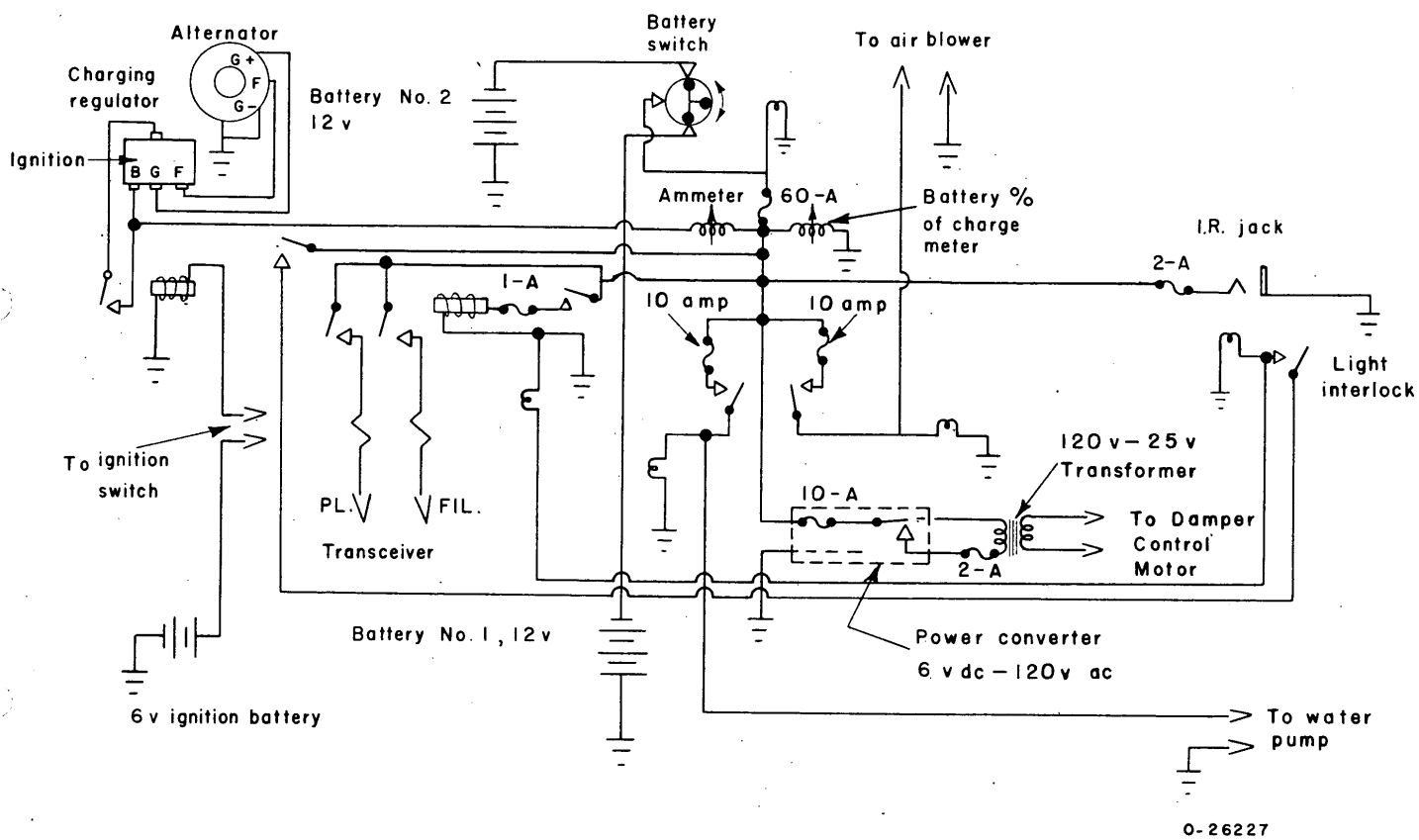
FIGURE 13A. ELECTRICAL SYSTEM SCHEMATIC
