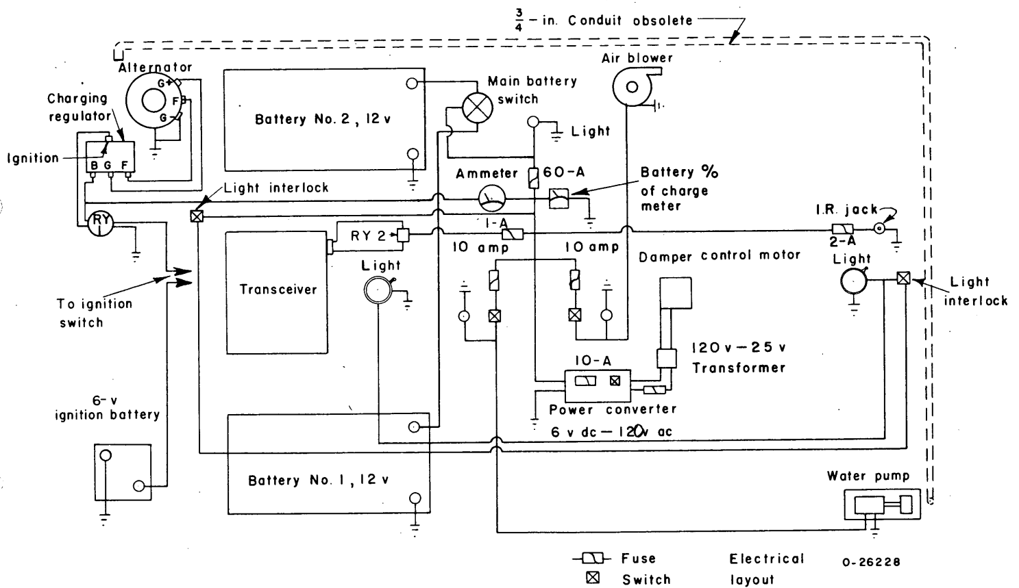
FIGURE 13B. ELECTRICAL SYSTEM PICTORIAL
