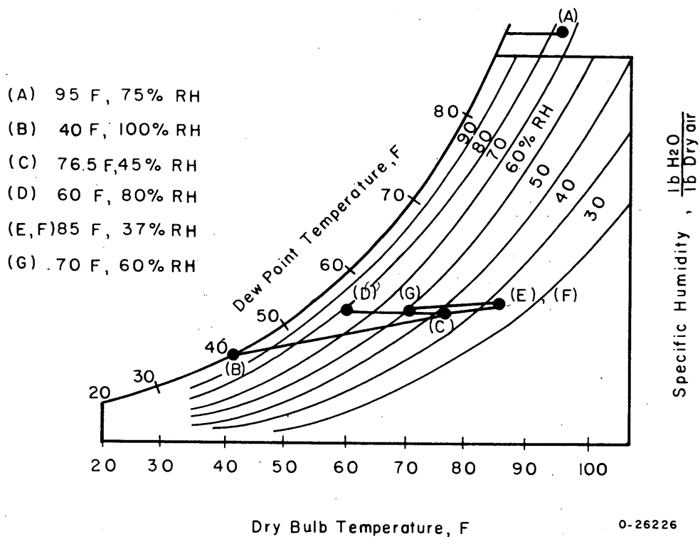
FIGURE 2. PSYCHROMETRIC CHART
