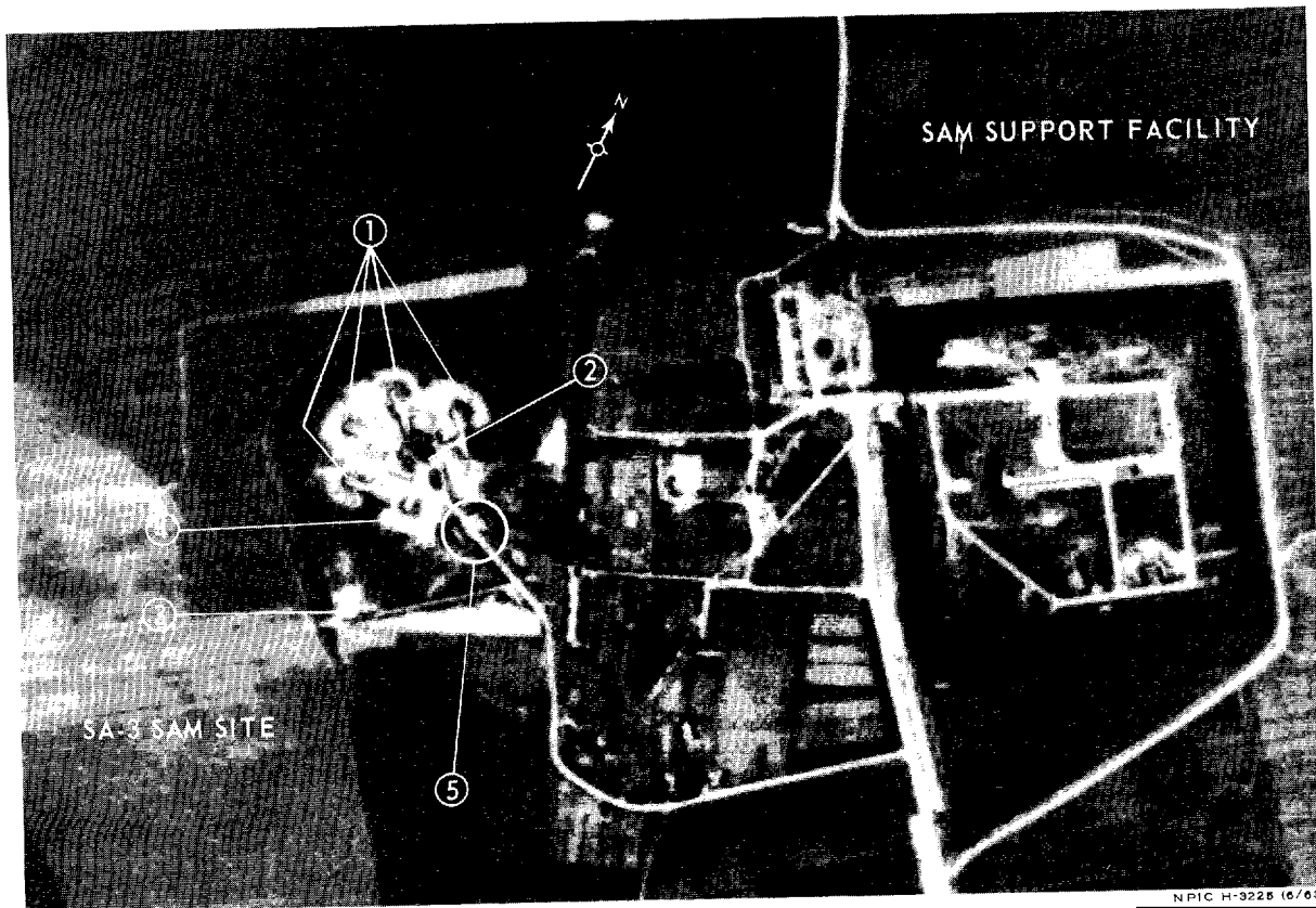
FIGURE 1. FACILITIES AND EQUIPMENT AT PRUZHANY MRBM COMPLEX SA-3 SAM SITE B16A, USSR
