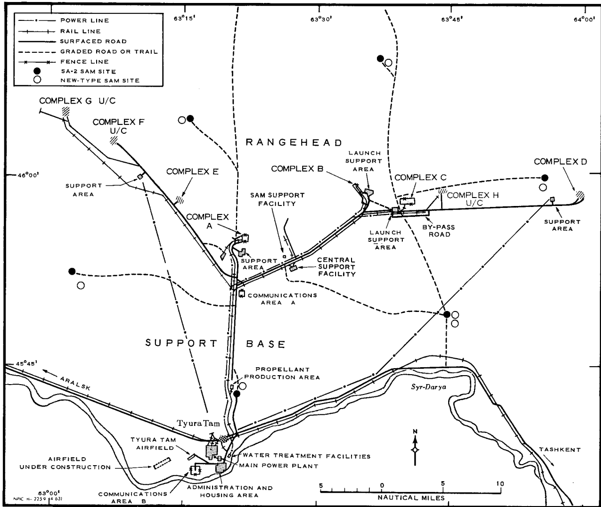
TYURA TAM MISSILE TEST CENTER (NEW ITEMS SHOWN IN RED)
