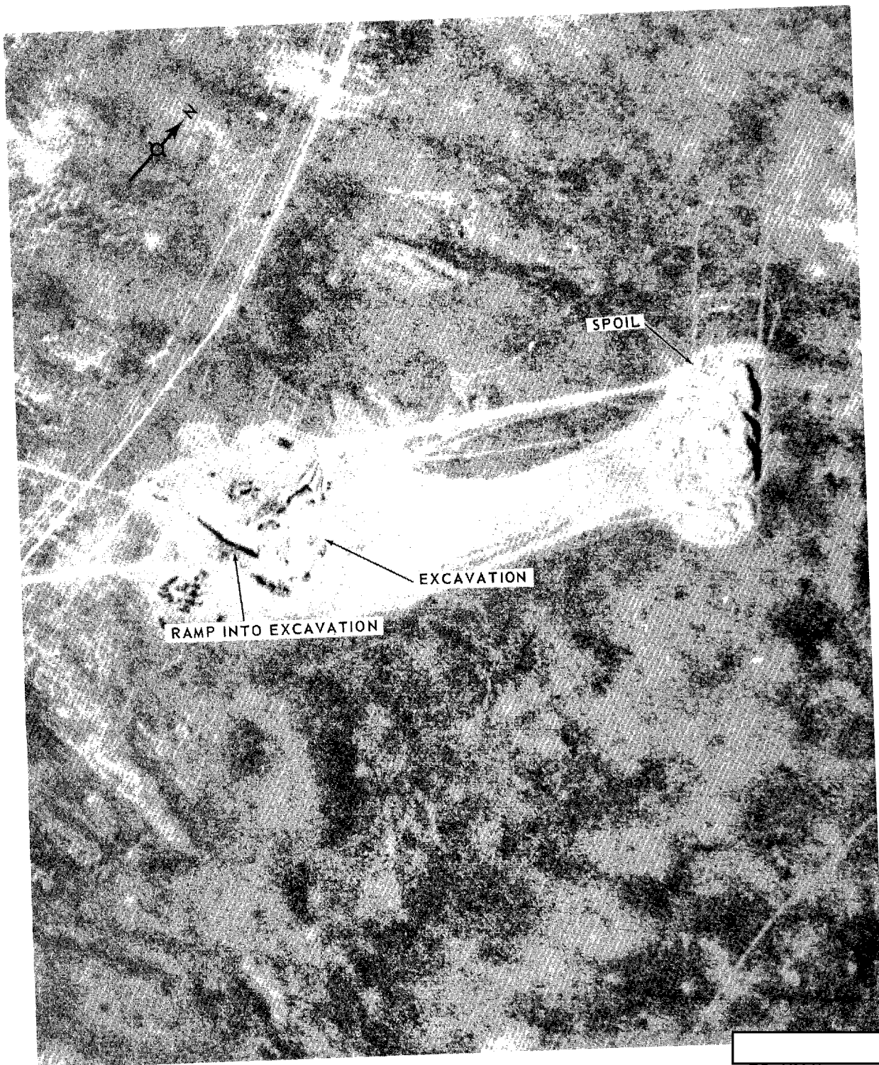
CONSTRUCTION ACTIVITY NEAR COMPLEX J, TYURATAM MISSILE TEST CENTER, USSR
