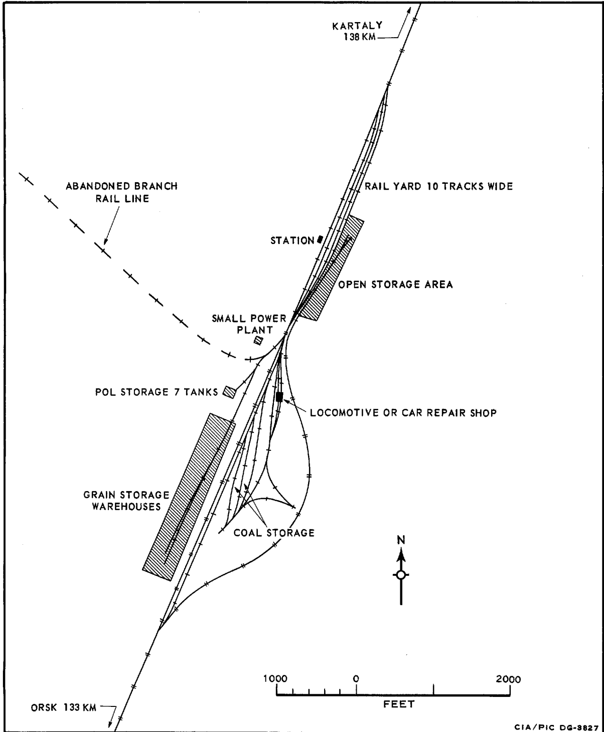
RAIL FACILITIES AT KRASNOYARSKIY (AYDYRLYA), USSR
