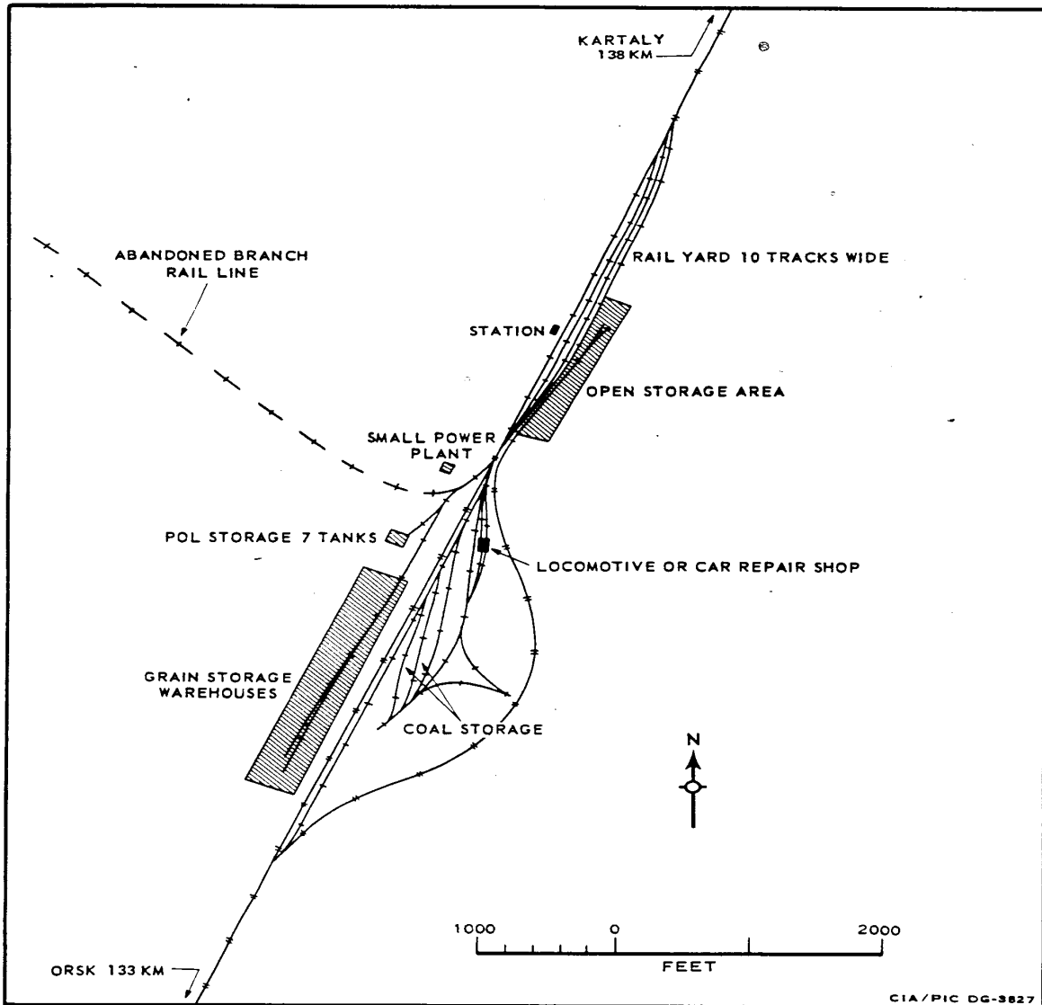
RAIL FACILITIES AT KRASNOYARSKIY (AYDYRL'YA), USSR
