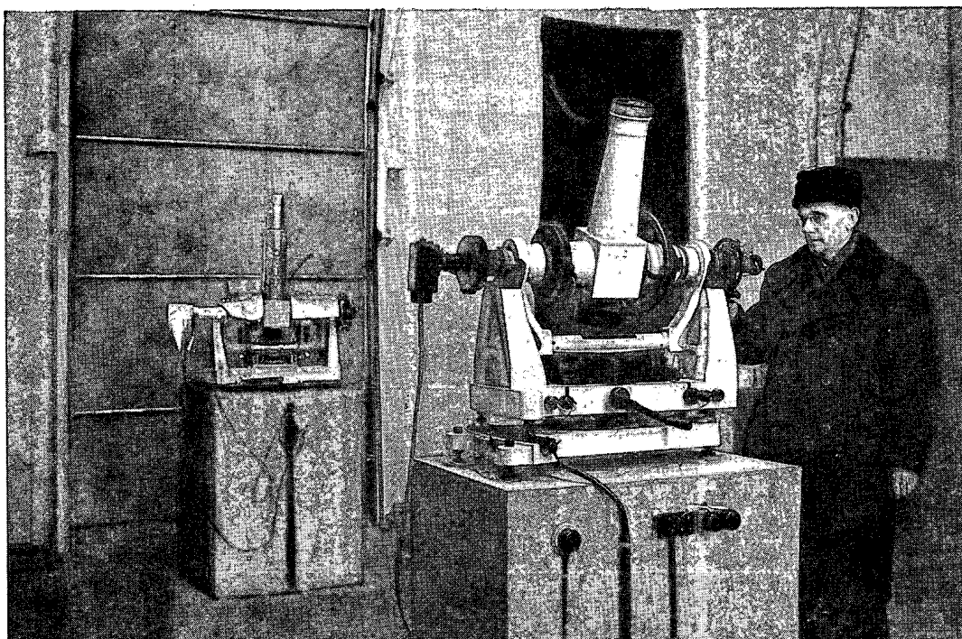
Time Service transit instruments with photoelectrical registration.
