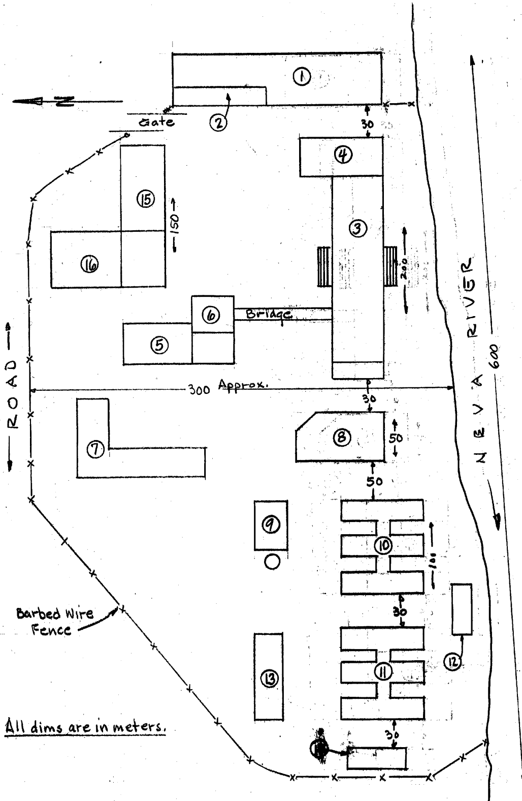
ENCLOSURE (B) Part 1 - Layout of GIPKh Institute
