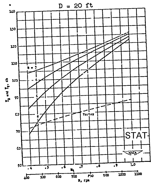
FIGURE 4.1.8 Same as Fig. 4.1.4, but for 8000 horsepower input.
