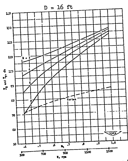
FIGURE 4.1.8 Same as Fig. 4.1.4, but for 8000 horsepower input.
