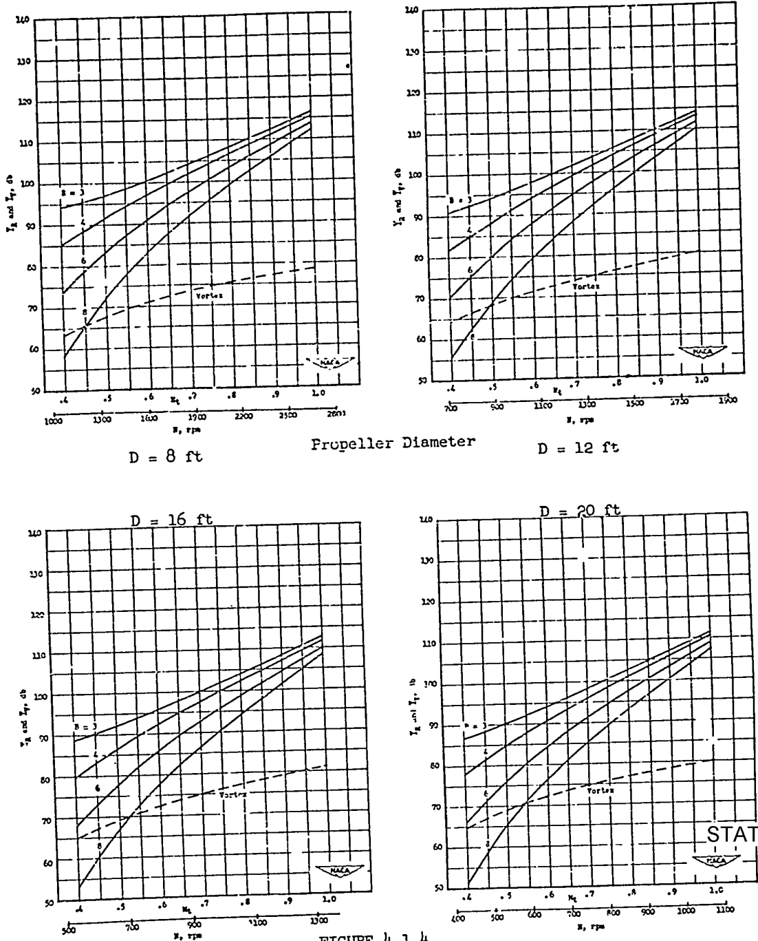
FIGURE 4.1.4 Overall rotational propeller sound pressure level, at 1000 horsepower input, as a function of tip Mach number and number of blades, for various propeller diameters (solid-line curves). The values are for 300 ft distance, in a direction 105° from the forward axis. To obtain the approximate acoustic power level of the propeller add 55 db to the result. The broken-line curves are estimated levels due to vortex noise. From Ref. (1.5).
