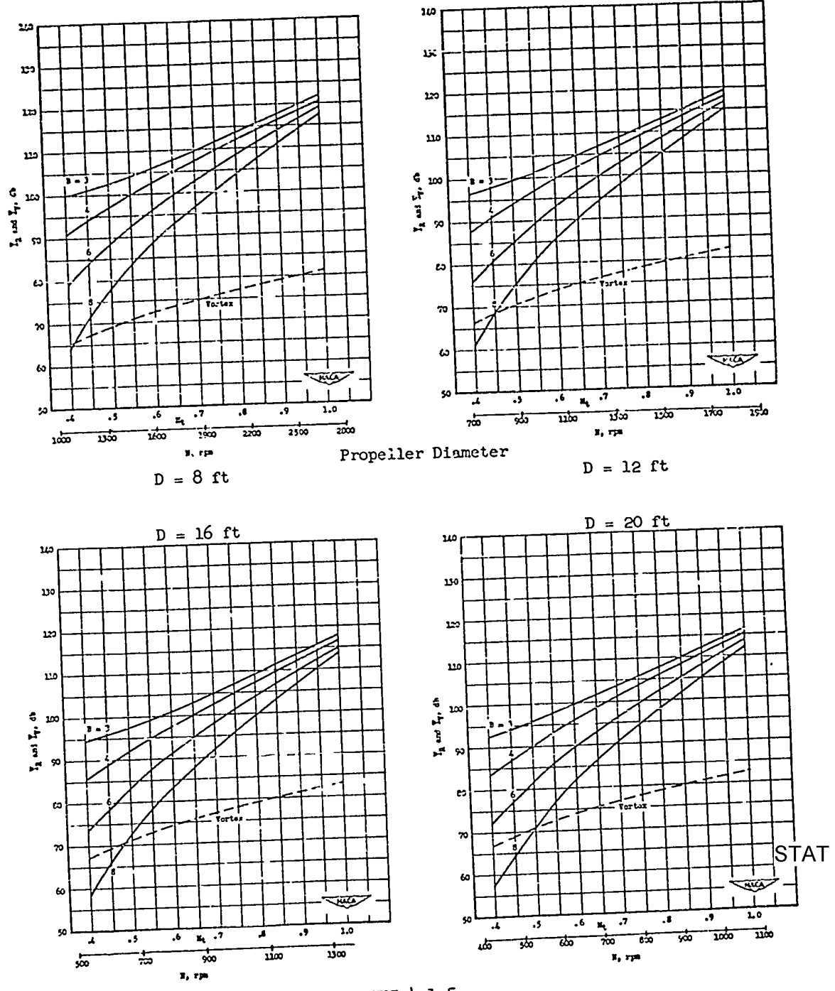
FIGURE 4.1.5 Same as Fig. 4.1.4, but for 2000 horsepower input.
