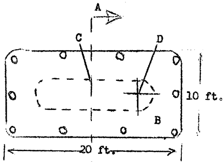
Sketch 3b: Plan view of working platform (see item 1 of Annex 2)
