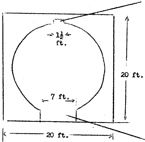
Sketch 3a: Cross section of air ducts (see item 3 of Annex 2)
