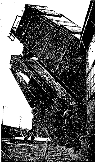
Tipping Plant for Freight Cars (used at the harbor of Wismar) For unloading the car is tilted by 60°
