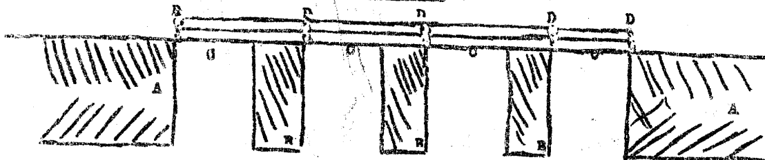
Bridge at South Exit of Pyatigorsk (Side View)
