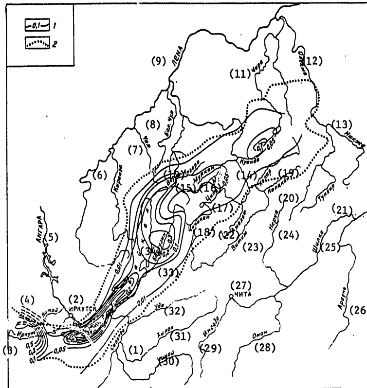
Figure 98. Map of the long-term seismic activity of Pribaykal'ye. Compiled by M. Novoselova, 1 -- isolines of the long-term component of the seismic activity; 2 -- boundary of the Baykal rift zone (according to Yu. A. Zorin, 1971)
