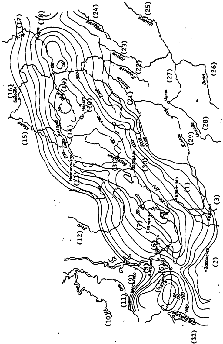
Figure 89. Map of the seismic vulnerability of Priбайка́l'ye. (Iz7, version 1)
