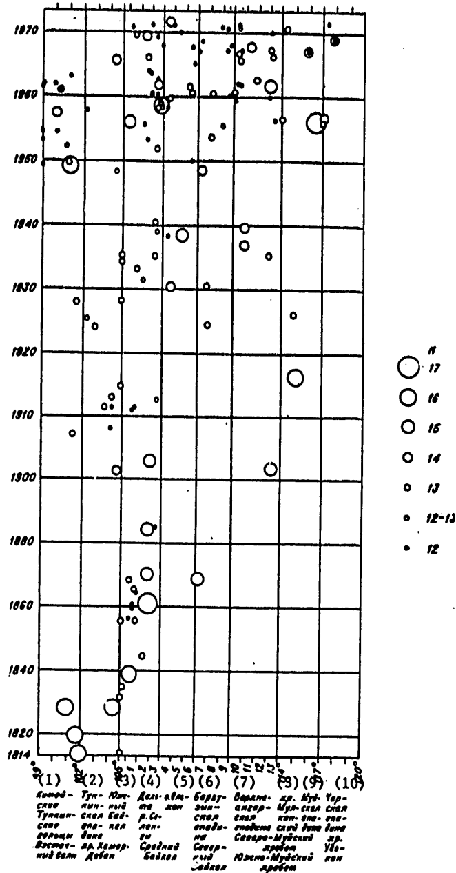
Figure 85. Time-space graph of the distribution of the strongest earthquakes of Pribaykal'ye (with M > 4 , K \geq 12 ) for the 19th to 20th centuries (in the projection of the rift system on the provisional axis according to Fig 84).
