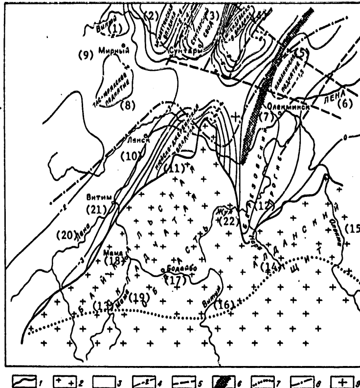
Figure 73. Schematic of the tectonic structure of the marginal structures of the Siberian platform of the vicinity of the Melichan earthquake of 9 October 1974.
