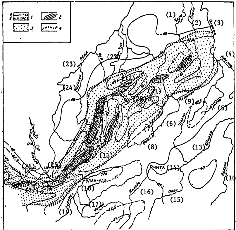
Figure 13. Schematic of the Deep Structure of Eastern Siberia. Compiled by Yu. A. Zorin
