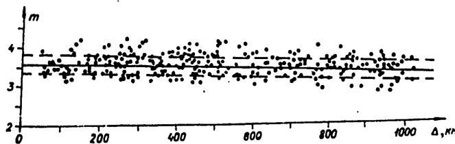
Figure 26. Results of determining the magnitude m by observations of earthquakes of the tenth energy class
