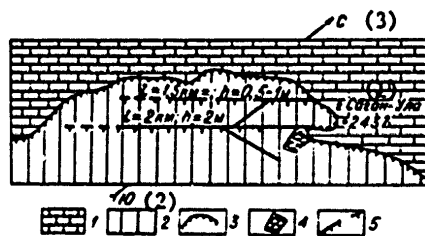
Figure 41. Plan of the Sarkhoy seismogenic structure.
