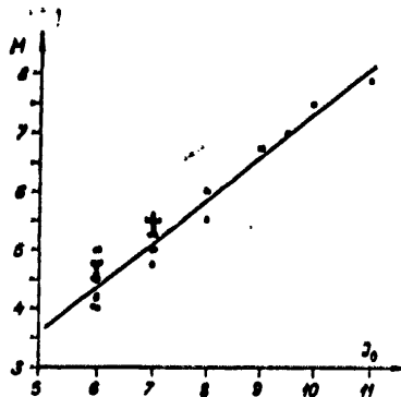
Figure 28. Determination of the relation of M and I_0 for the Pribaykal'ye earthquake
