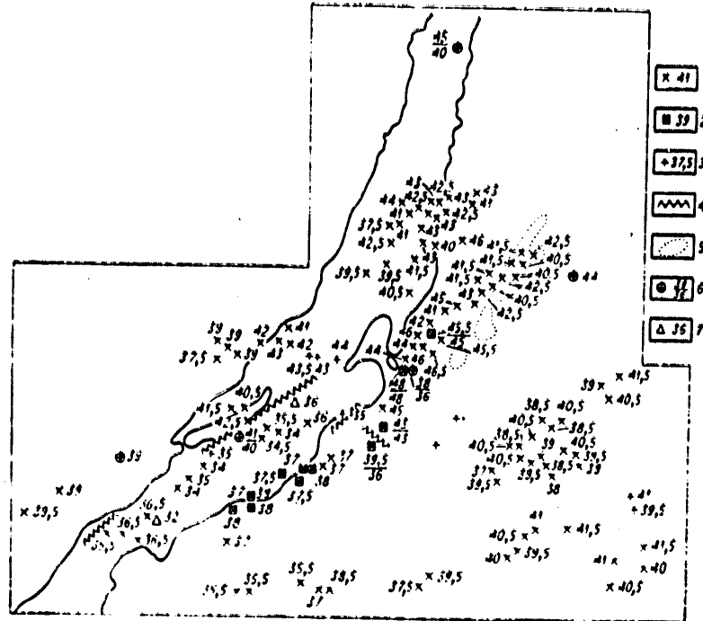
Figure 105. Depths with respect to the mantle surface in the Baykal region and Transbaykal according to the deep seismic sounding data and observations of earthquakes.
