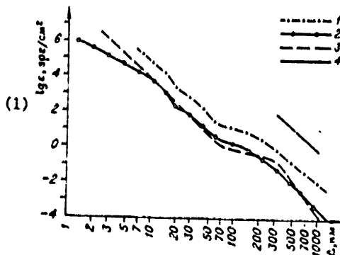
Figure 19. Graphs of the damping of the energy flux density. 1 -- constructed by the T. G. Rautian procedure; 2 -- constructed using the function F_p(\Delta) ; 3 -- calibration curve for the T. G. Rautian nomogram; 4 -- determined by the difference method.
