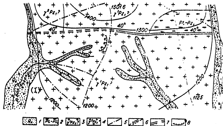
Figure 59. Schematic of the geological structure of the landslide-landslip section of Tanga.
