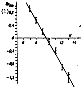
Figure 21. Function \delta n_{eff}(K)
