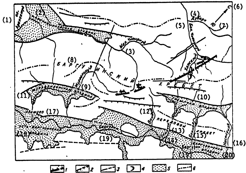
Figure 49. Plan of the Malochivyrkuyskaya structure.
