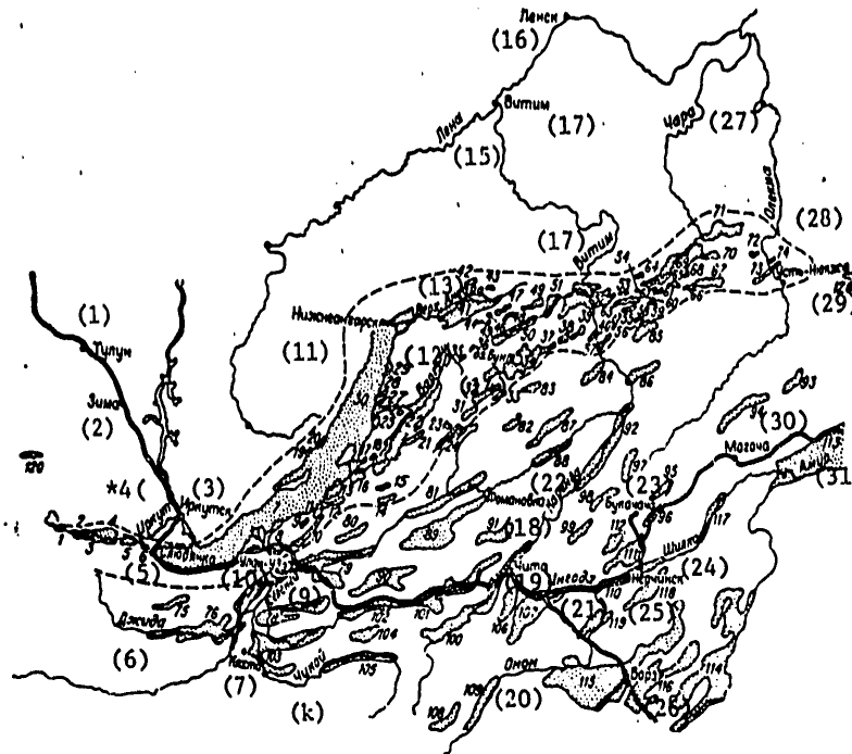
Figure 104. Schematic of the arrangement of the most important basins of the epiplatform orogenic belt of Eastern Siberia. The dotted line denotes the boundary of the Baykal rift zone. Compiled by R. Kurushin, S. Lastochkin.
