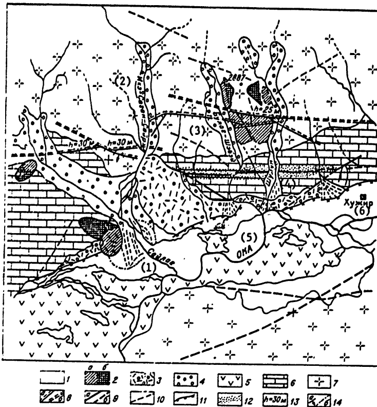
Figure 44. Plan of the seismogenic Shulun structure.
