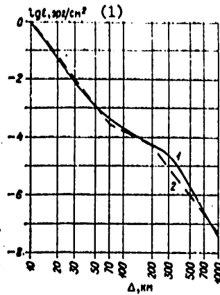
Figure 23. Comparison of the damping graph of the energy flux density for Pribaykal'ye (2), the calibration curve for the T. G. Rautian nomogram (1)
