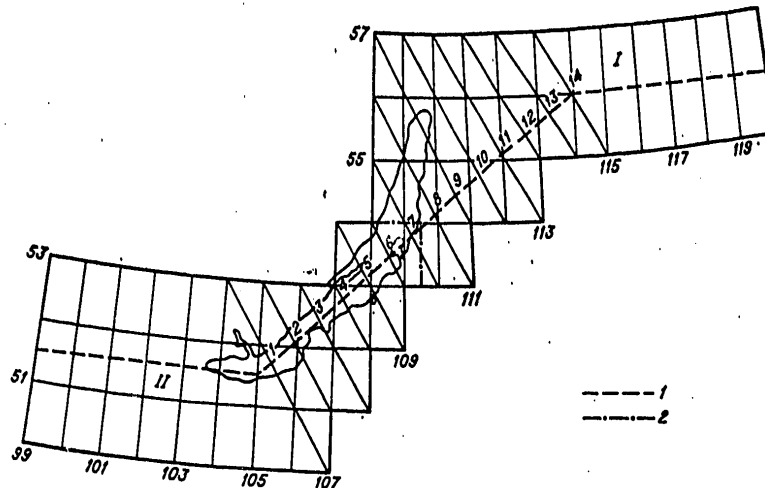
Figure 84. Schematic of the provisional axis of the Baykal rift zone. 1 -- provisional axis of the rift zone; 2 -- provisional boundary separating the northeastern (I) and southwestern (II) parts of the zone.
