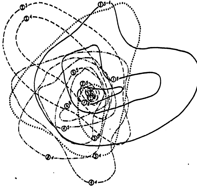
Figure 27. Map of the combined isoseisms of earthquakes with M=5.3-5.5 . The numbers: in the circles, the earthquakes numbers (see Table 8); outside the circles, the force indication
