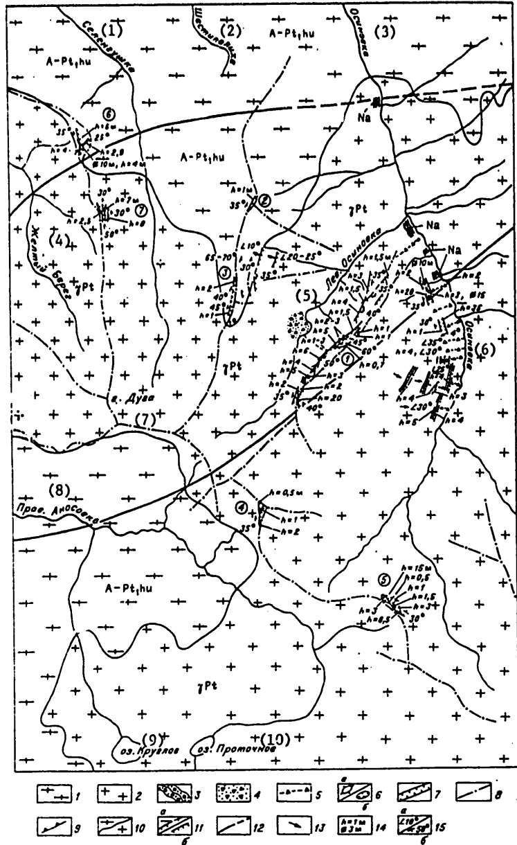
Figure 54. Plan of the basic structural field, Compiled by S. Lastochkin and A. Abalakov.
