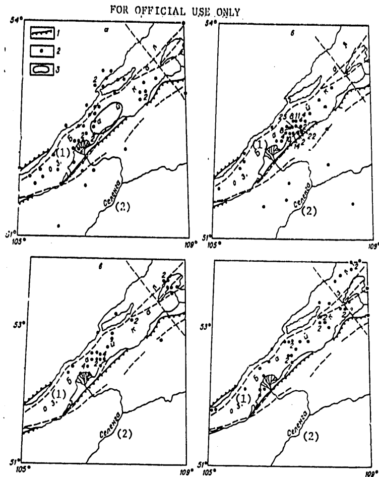
Figure 94. Analysis of the epicentral field in the vicinity of Central Baykal by the data on earthquakes with K \geq 10 for 1952-1970
