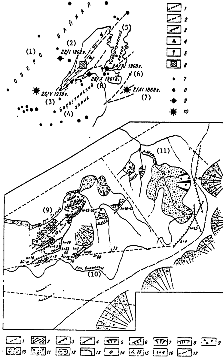
Figure 47. Plan of the central part of the Svyatonosskaya structure. Compiled by A. Abalakov. [See legend and key on p 169]
