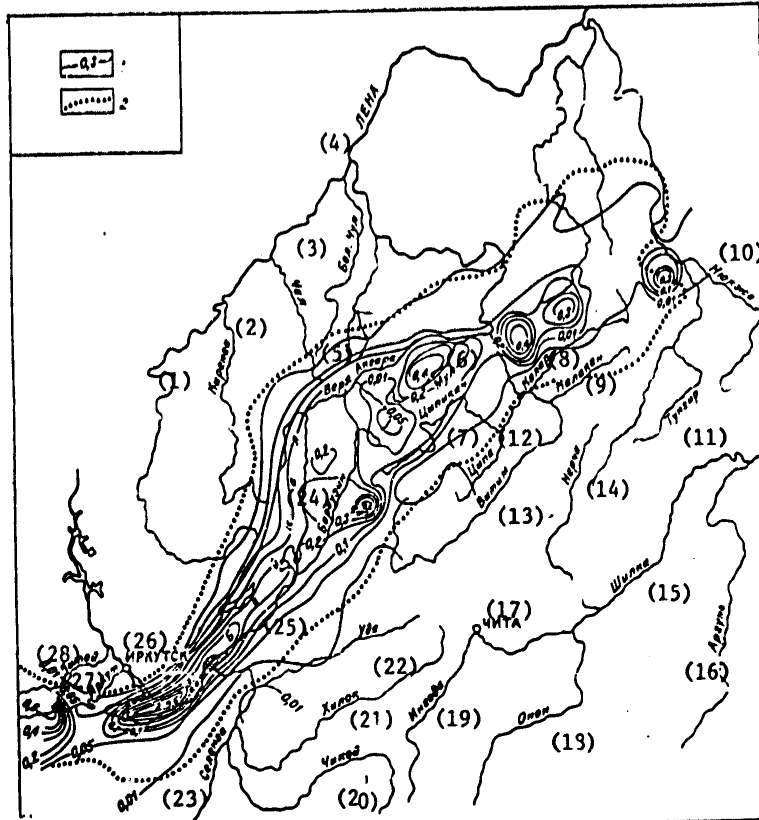
Figure 99. Map of forecasting the total seismic activity (long-term and short-term component) of Pribaykal'ye. Compiled by M. Novoselova and L. Bogatova.
