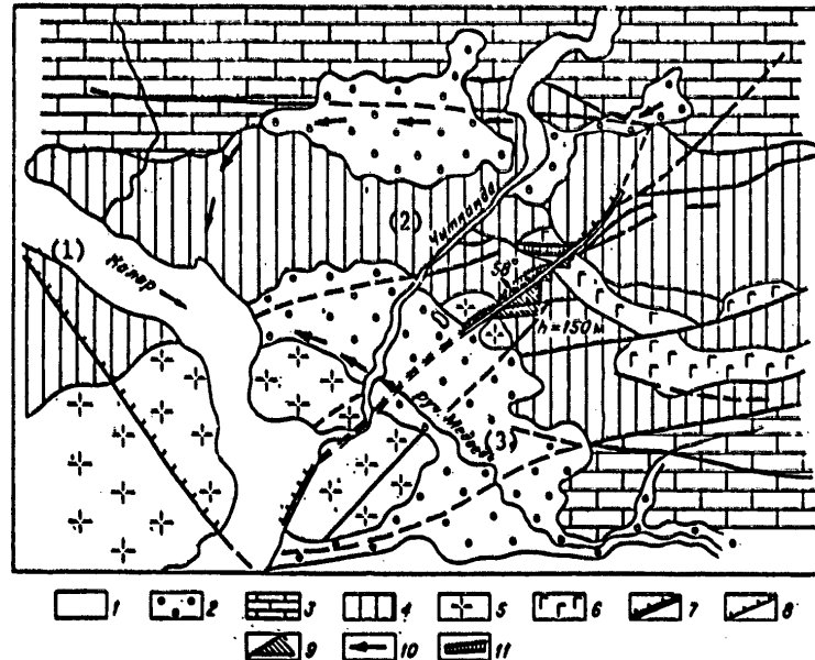
Figure 40. Plan view of the Medved' seismogenic structure. Compiled by M. Dem'yanovich.
