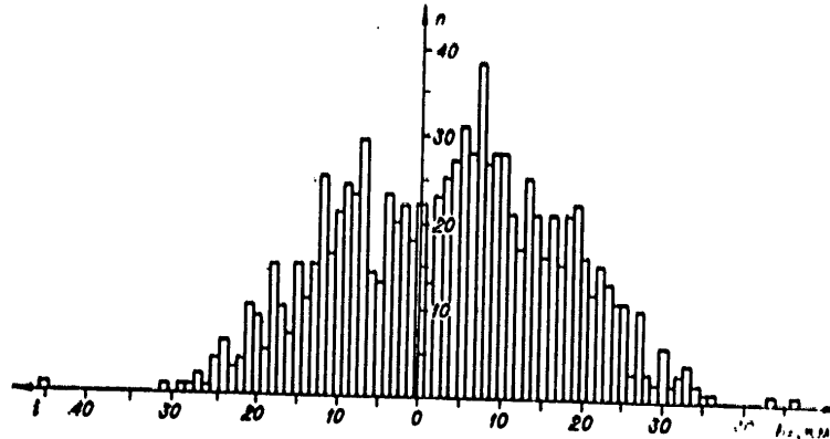
Figure 81. The distribution of the depths of centers of Pribaykal'ye earthquakes in 1967 in accordance with the observations of the \bar{S} waves (n is the number of determinations)
