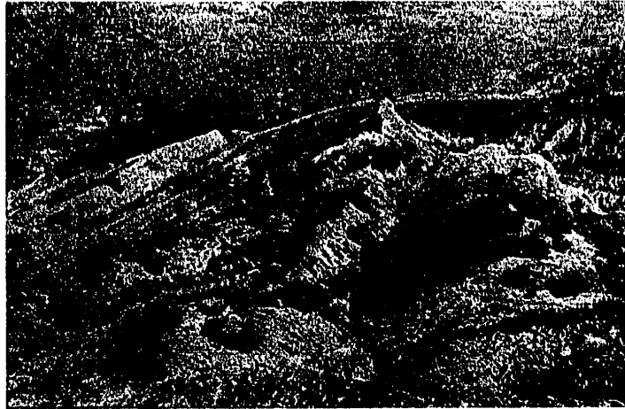
Figure 51. Seismogenic faults on the northwest side of the Bol'sherechenskaya basin. Amplitude of vertical displacement with respect to the fracture in the center of the photograph is 8 meters. In the background is the Bol'sherechenskaya basin. Photograph by A. Abalakov.
