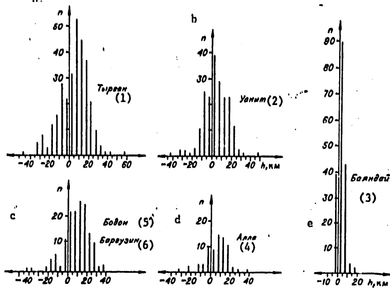
Figure 80. Earthquake distribution with respect to depths. a-d -- by the observations of the longitudinal head waves P, e -- by reflected transverse waves
