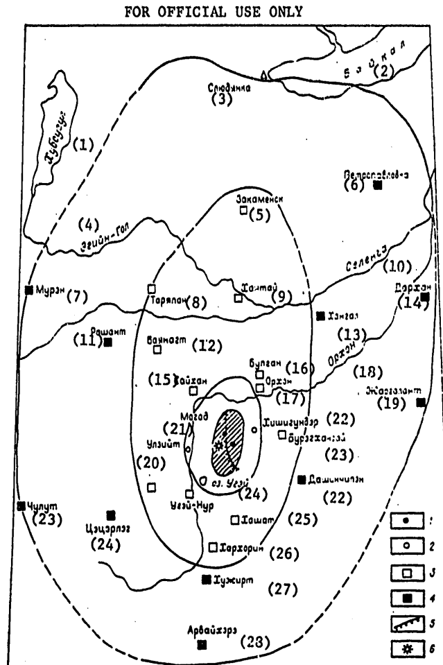
Figure 10. Isoseismal map of the Mogodskoye earthquake of 5 January 1967. Compiled by S. Khil'ko and I. Balzhinnyam.
