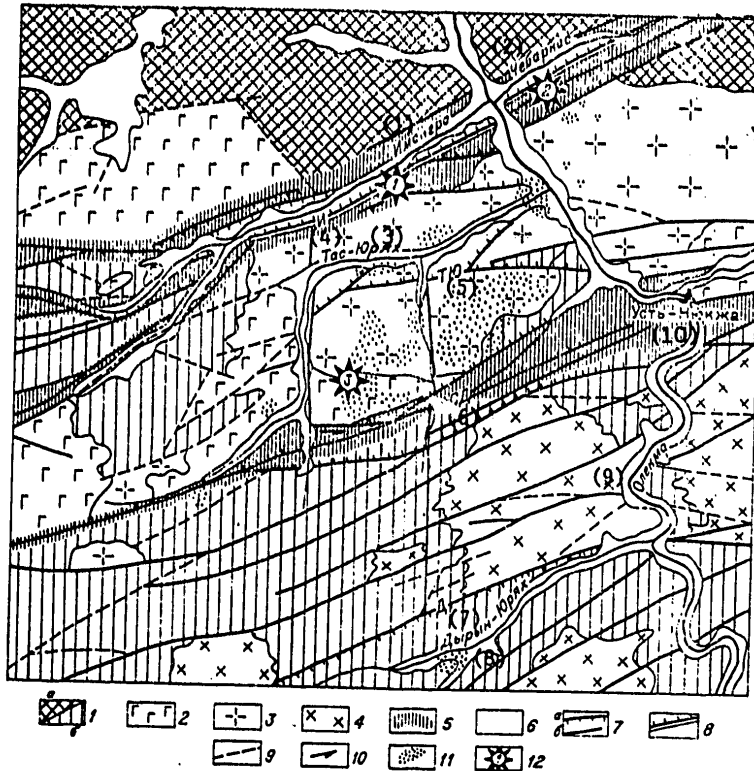
Figure 71. Seismogeological diagram of the epicentral region of the Tas-Yuryakhskiy earthquake on 18 January 1967. Compiled by S. Khil'ko.
