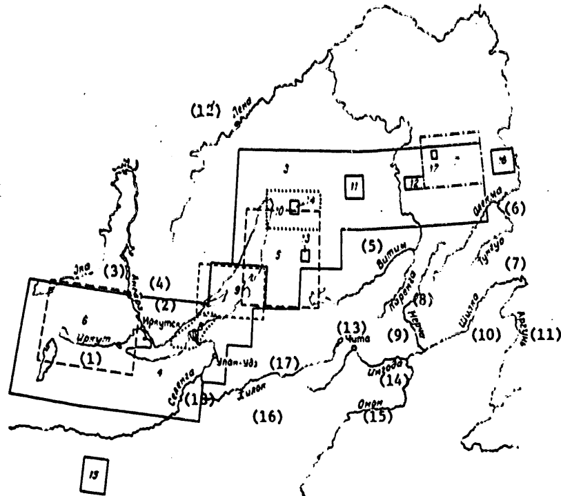
Figure 82. Schematic of the regions of calculation of the earthquake recurrence rate graphs. The numbers correspond to the numbers of the regions in Table 13.
