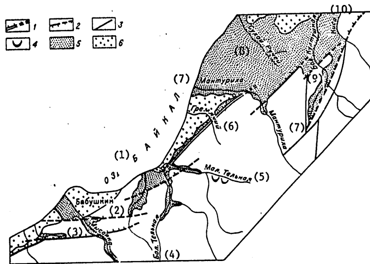
Figure 56. Plan of the Manturikhinskaya [Manturikha] structure. Compiled by A. Abalakov.
