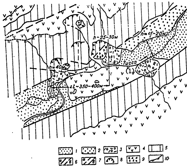
Figure 43. Visual plan (with refinements by aerial photograph) of the Dugaray structure.
