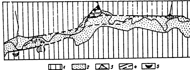
Figure 45. Plan of the proposed seismogenic Tustuk structure. Compiled by V. Nikolayev.
