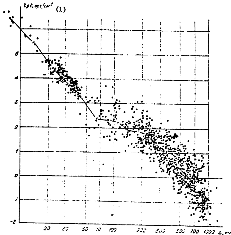
Figure 17. Summary graph of the damping of the energy flux density for Pribaykal'ye constructed by the T. G. Rautian procedure
