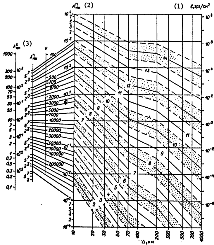
Figure 24. Nomogram taking into account the seismic wave damping as a function of earthquake energy
