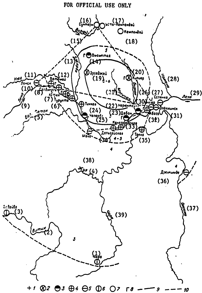
Figure 72. Isoseismal map of the Melichanskiy [Melichan] earthquake of 8 October 1974, Compiled by A. D. Abalakov, T. M. Kozyrev. 1 -- epicenter according to the instrument data; 2 -- force 5-6; 3 -- 5; 4 -- force 5; 5 -- 4; 6 -- force 3; 7 -- not felt; 8 -- populated areas where the roar was heard; 9 -- isoseisms; 10 -- examination route; The numbers indicate the force period, [See key on p 219]
