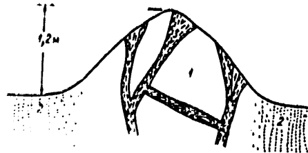
Figure 6. Earth Spout mound in the Khaik Avalanche in the Ya man River Valley 1 -- pale yellow structureless loam; 2 -- the same with restored loess structure; 3 -- dark brown loam with flow texture. The mound was formed on 10 July 1949 and it was discovered on 21 October 1968.
