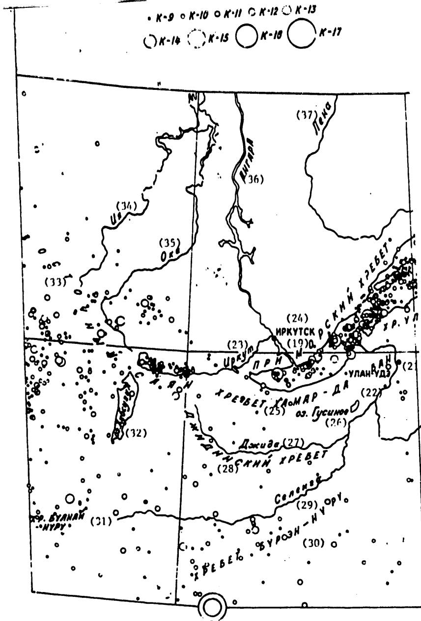
Fig 74. Map of the earthquake epicenters of Pribaykal'ye for 1962-1971 [See key on p 226]
