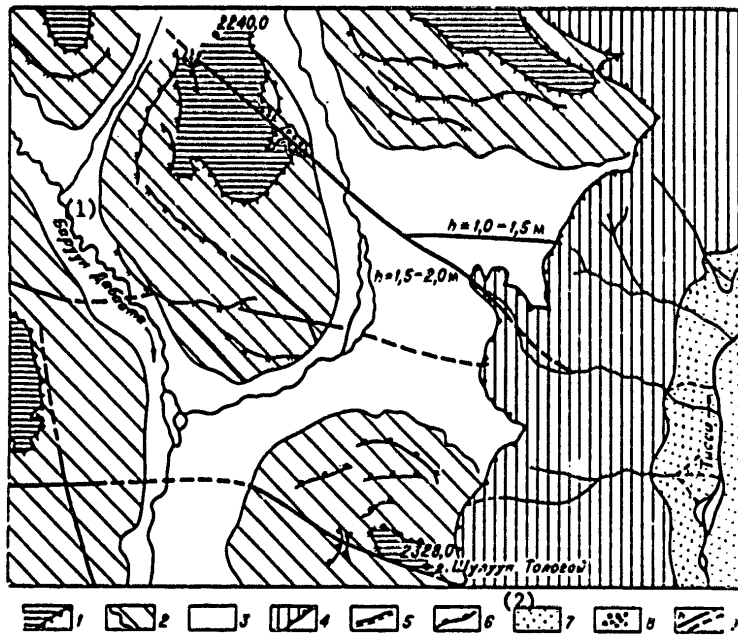
Figure 42. Schematic of the Tology structure. Compiled by M. Dem'yanovich.
