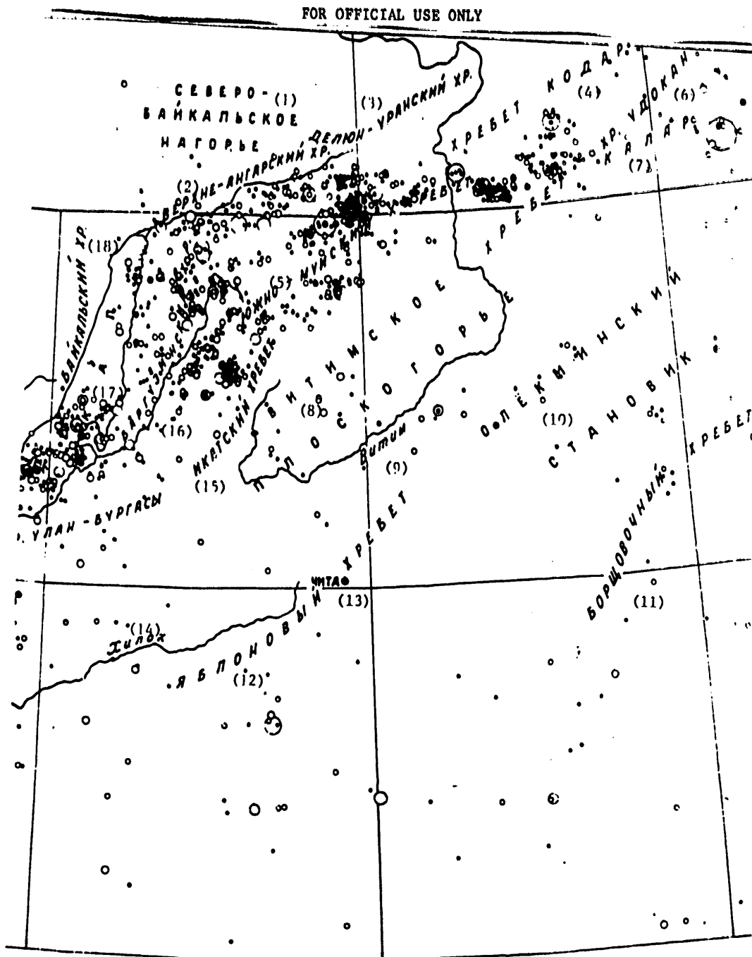
(K-9). The numbers in the notation correspond to energy classes of the earthquakes. [See key on p 226]
