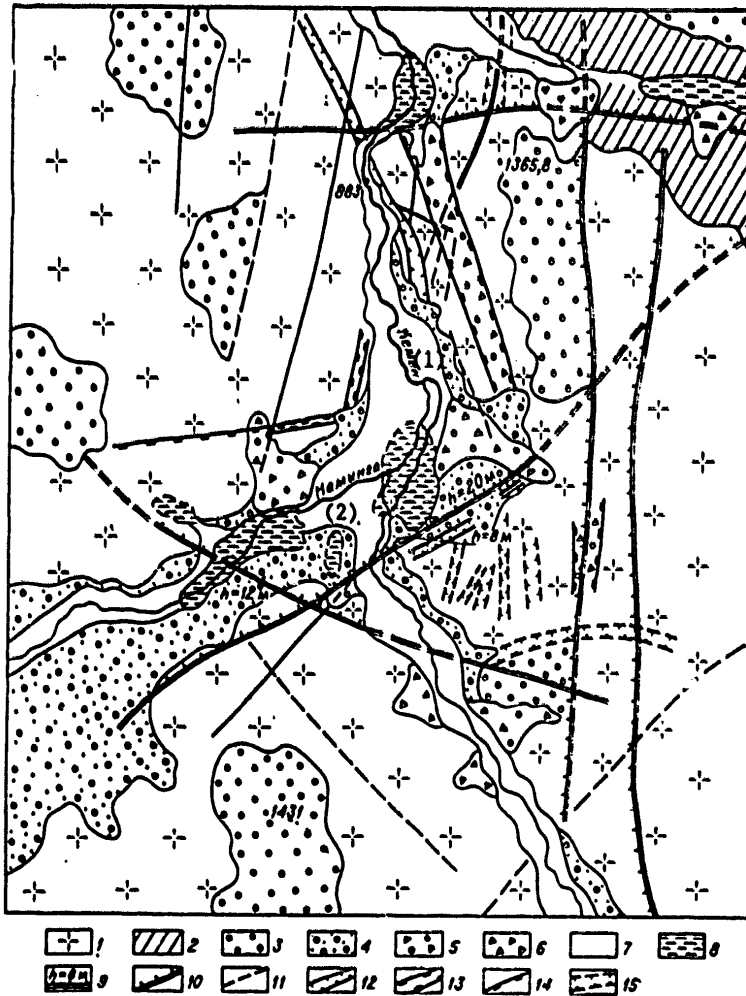
Figure 39. Seismogeological schematic of the Kemn basin. Compiled by M. Dem'yanovich.
