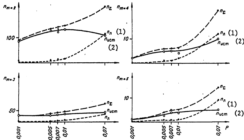
Figure 93. Grouping of weak earthquakes for various values of the probability of random occurrence of an event. n_E is the total number of isolated groups; n_{true} is the number of true groups; n_f is the number of false groups; m is the number of groups (the numbers 2, 3, 4, 5 are the number of shocks in the group)
