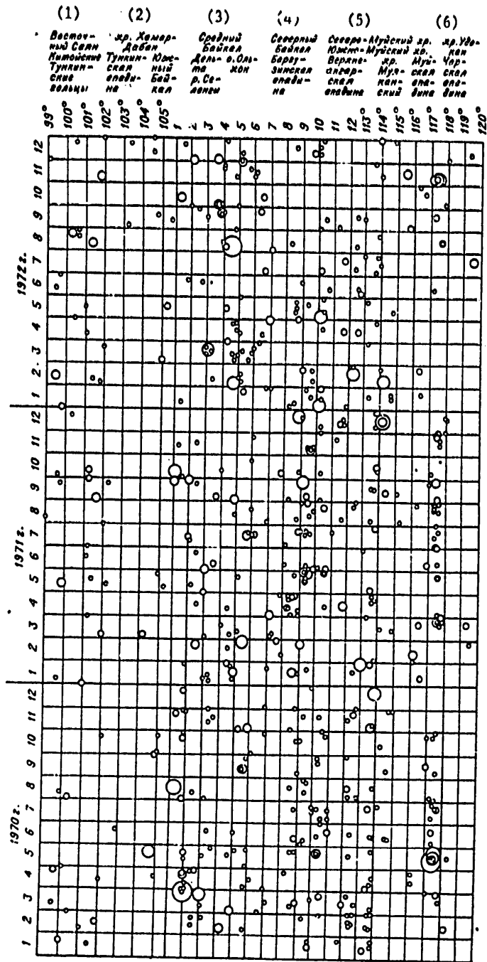
Figure 86. Time-space graph of the earthquake distribution for Pribaykal'ye [See key on p 250]
