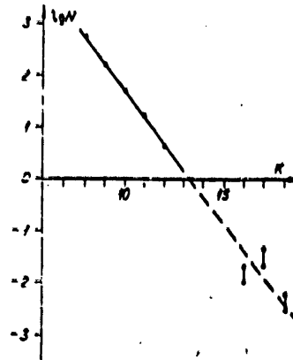
Figure 83. Graph of the recurrence rate of earthquakes in the Baykal rift zone (the dark circles are according to the instrument data, and the light circles, according to the data on the paleoseismodislocations).
