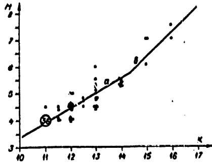
Figure 29. Relation between M and K. a -- K=1.8+4M ; b -- K=8+1.1M . The number "36" indicates that 36 earthquakes have values of K=11 and M=4 .
