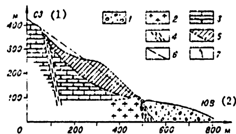
Figure 37. Geological-geomorphological section through the axial part of the seismogravitational rockslide on the southeast slope of the Adyanskaya ridge. Compiled by R. A. Kurushin
