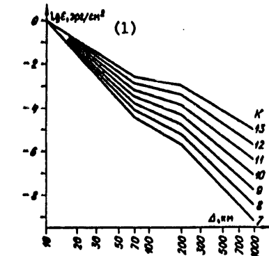
Figure 22. Damping curves of the energy flux density for earthquakes of different energy classes
