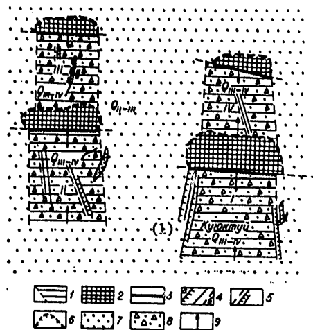
Figure 57. Morphometric schematic of the graben-like Kuyuktuy structures. Compiled by S. Lastochkin. 1 -- graben-like closed basins; 2 -- outliers; 3 -- transverse fault; 4 -- longitudinal faults, reliable (a) and proposed (b); 5 -- benches of the terraced areas; 6 -- granite outcrops; 7 -- Middle to Upper Pleistocene sand and sandy loam deposits; 8 -- bottoms of the basins made from Pleistocene-Holocene coarse sediments; 9 -- direction of removal of loose material; I-IV -- numbers of bay basins.
