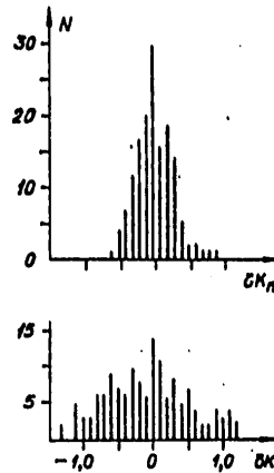
Figure 25. Histograms of deviations from the mean when determining the energy classes by the nomograms presented in Fig 24, and by the T. G. Rautian version
