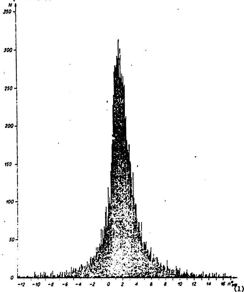
Figure 18. Distribution N(n_{eff}^*) for the damping law of the seismic waves as a function of the Pribaykal'ye earthquakes (for the difference method).
