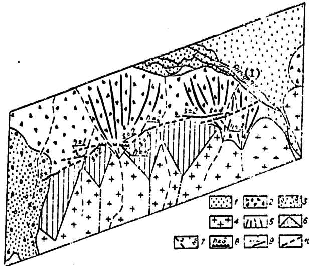
Figure 31. Schematic of the northeastern flank of the Yanchukanskaya structure. Compiled by R. A. Kurushin
