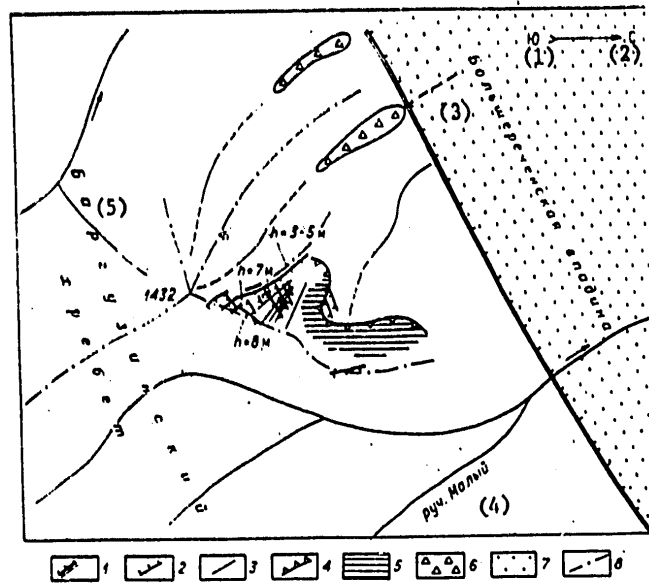
Figure 50. Visual plan of the Bol'sherechenskaya structure. Compiled by A. Abalakov.
