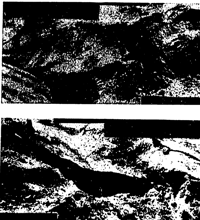
Figure 1. Seismogravitational or Gravitational-Seismic Tectonic Structure of Akiba (the Greater Caucasus), photograph by V. M. Zhilkin
