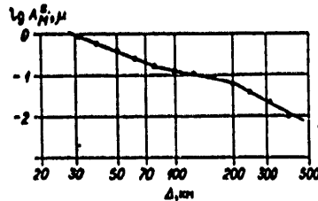
Figure 20. Graph of damping of maximum amplitudes, soil displacements constructed by the method of "successive reproduction"
