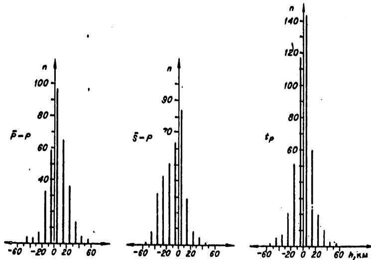
Figure 79. Earthquake distribution in Pribaykal'ye according to center depths h using the differences in times of arrival of the \bar{P} and \bar{S} waves and the head waves P and absolute travel times of the head waves P ( t_p ) at individual stations, n is the number of cases.
