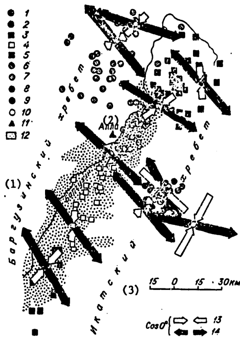
Figure 14. Orientation of the Stress Axes in the Centers of Earthquakes of the Barguzin District 1-10 -- epicenters of earthquakes belonging to groups Nos 22-31 respectively in Table 3; 11 -- seismic station; 12 -- basin region; 13-14 -- compressive and tensile stresses, respectively, indicated for each group in the example of one of the earthquakes (the length of the arrows is proportional to the cosine of the slope angles of the axes to the horizontal plane). Key: 1. Barguzin ridge; 2. Alla; 3. Ikatskiy ridge
