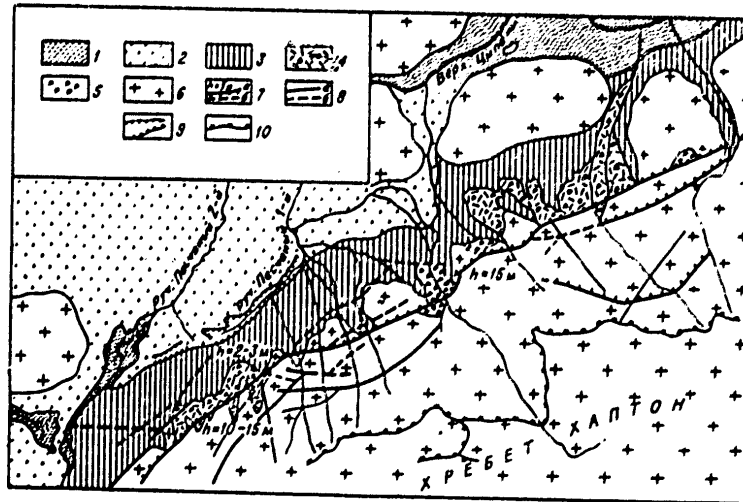
Figure 52. Plan of the Khapton seismogenic structure. Compiled by M. Dem'yanovich.
