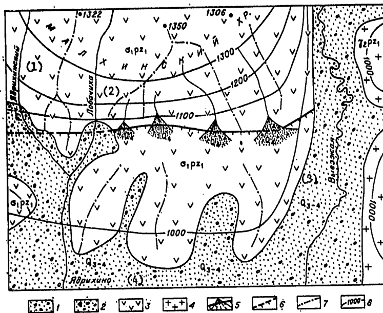
Figure 58. Diagram of the geological structure of the Yadrikha seismogenic structure.
