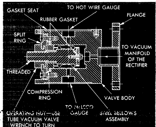
FIG. 20 Cross-sectional view of three-way type vacuum valve.
