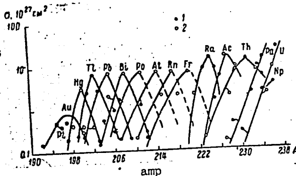
Figure 4: Distribution curves of the yield of isotopes of different elements according to mass number in uranium fission with 660 Mev protons. 1 - experimental values; 2 - interpolated values.
