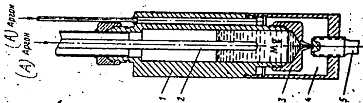
Figure 2: Diagram of the device for obtaining metal drops. 1 - body; 2 - thermocouple; 3 - headpiece; 4 - chamber; 5 - plug; (A) Argon.
