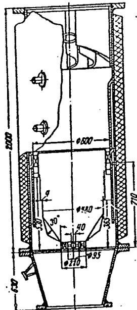
Fig. 1. Combustion chamber.
