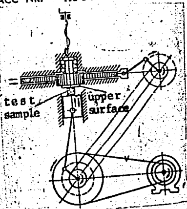
Fig. 1. Elastic-materials testing machine
