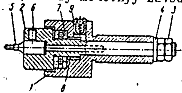
Рис. 2. Fig. 2. The combined method of broaching an inside hexagon: (1) holder, (2) die, (3) nuts, (4) disc, (5) die, (6) screw, (7) thrust bearing, (8) bronze bush, (9) lubricating valve.
