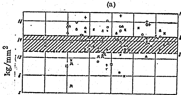
Fig. 1 -- Dependence of the ultimate strength of alloys on the pouring temperature and casting depth.
