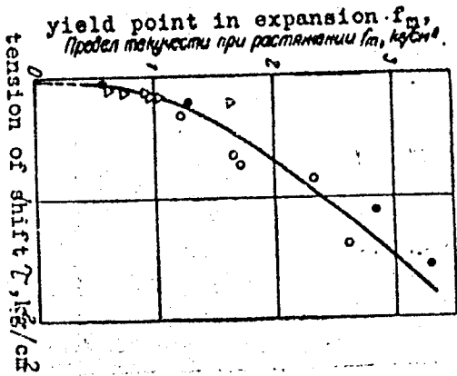
Figure 6: Relationship between the shear tension at a rate gradient of \dot{\gamma} = 0.01 1/sec and yield point in expansion for rubber mixtures in the case of \dot{\gamma} = 0.067 1/sec: ● - mixture for rubber articles, ○ - mixtures for rubber footwear, △ - model mixtures based on SKB.
