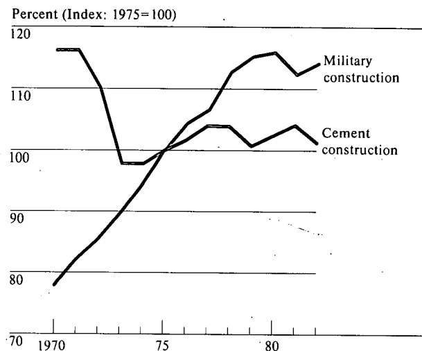
Figure 3 Trends in Cement Production and Military Construction, 1970-82
