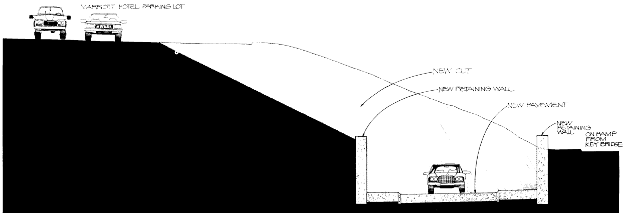
ALTERNATIVE D NEW OFF RAMP TO ROSSLYN CIRCLE FROM INBOUND PARKWAY WITH R.O.W. PURCHASE
