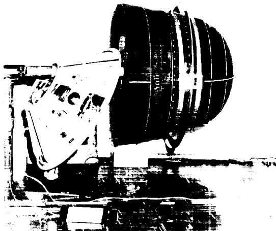
Thrust Cone Ejected
