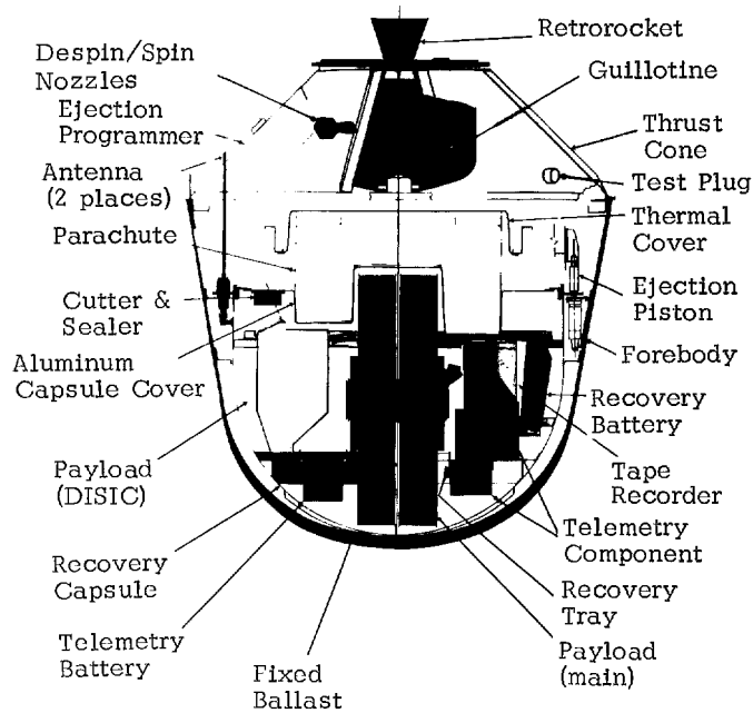
— J-3 System —
