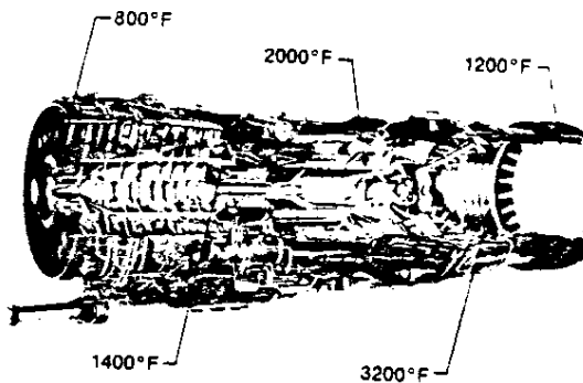
Figure 2. J58 Flight Temperature
