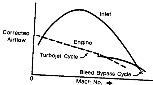
Figure 3. Inlet and Engine Air Flow Match.
