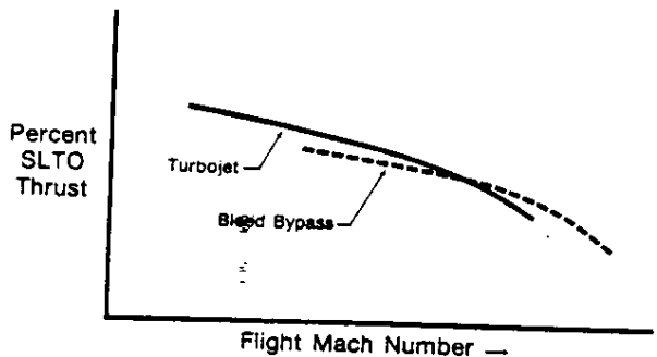
Figure 4. Net Thrust Comparison - Bleed Bypass Cycle vs Turbojet Cycle.
