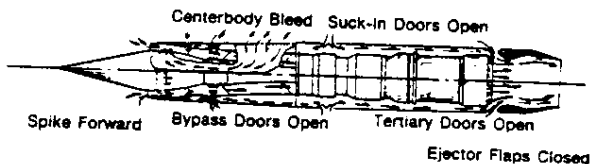
Figure 6. Air Flow Patterns - Static Aircraft
