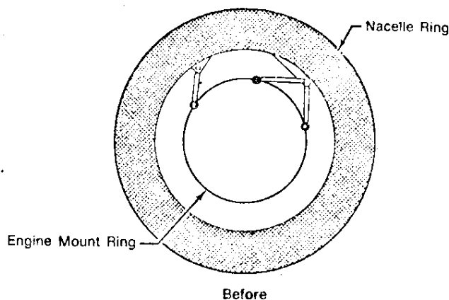
Figure 7. Engine Mount
