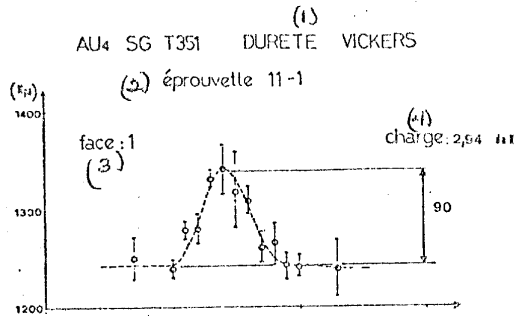
Fig. 7. Hardnesses measured on the two sides of light-alloy test piece 11-I, after test. KEY: (1) Vickers hardness. (2) Test piece 11-I. (3) Side. (4) Load. (5) Distance to the marked end.
