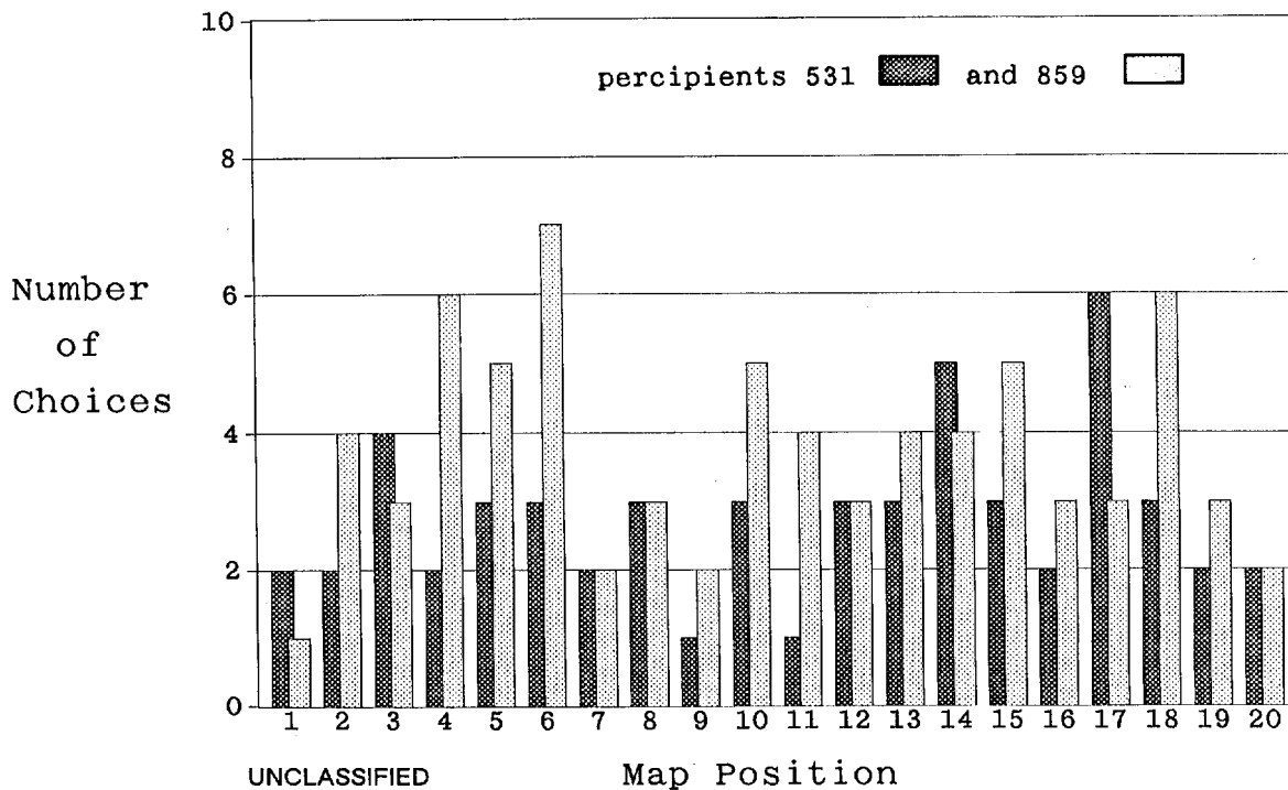
FIGURE 6 CHOICE HISTOGRAM
