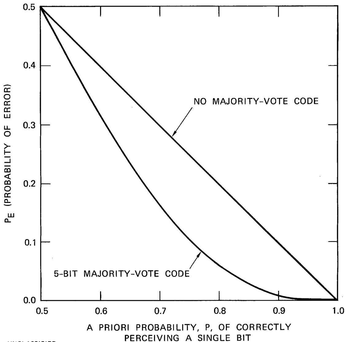
FIGURE 3 (U) PROBABILITY OF ERROR, P_E , WITH AND WITHOUT USE OF A SIMPLE 5-BIT MAJORITY-VOTE CODE
