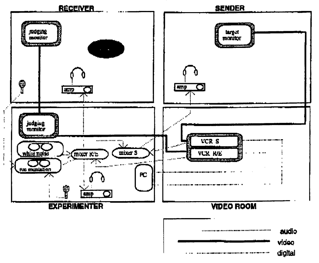
Figure 2. Audio, video, and digital communications layout. This design isolates the audio and video (a/v) paths for S and R/E to avoid introducing sensory cuca. The only direct connection between S's and R's a/v systems is the output of the audio mixer into the input of the S audio mixer.
