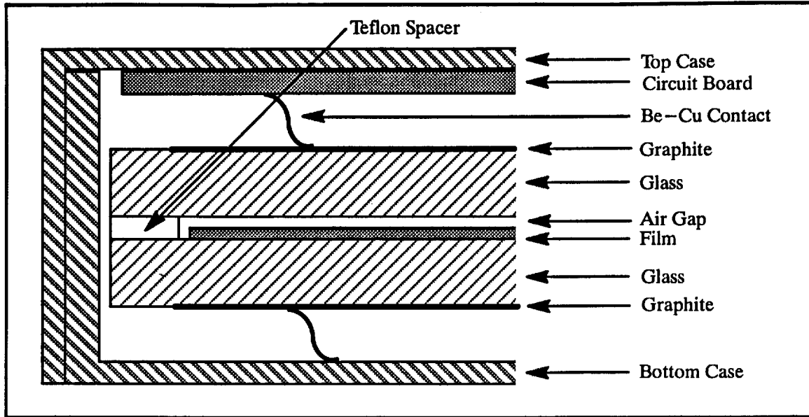
Figure 4. Cross-Section of the Detector (Not to Scale).
