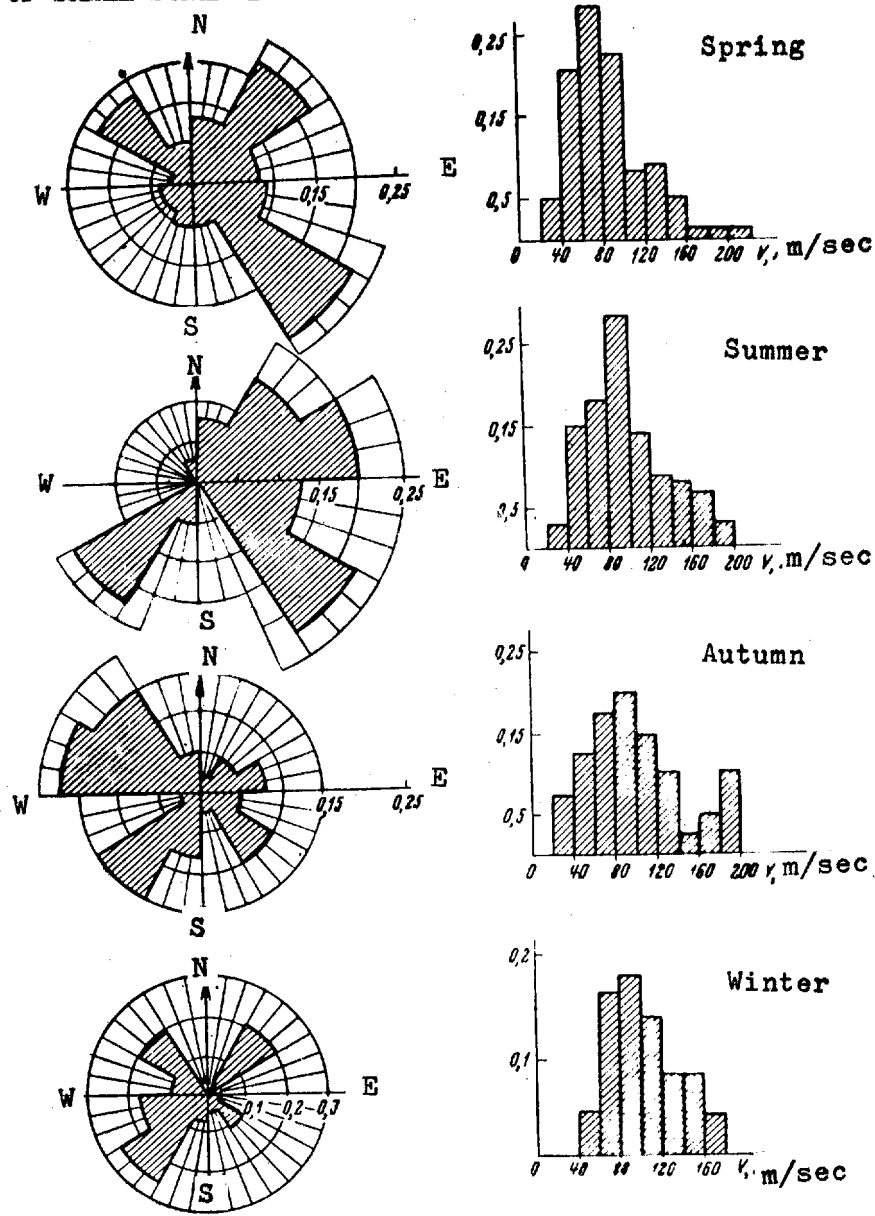
Fig. 5. Histograms of the magnitude of the velocity and direction of drifts in the E layer for different times of the year. The relative number of cases n_i / \sum n_i are plotted on the y-axes and along the radii.
