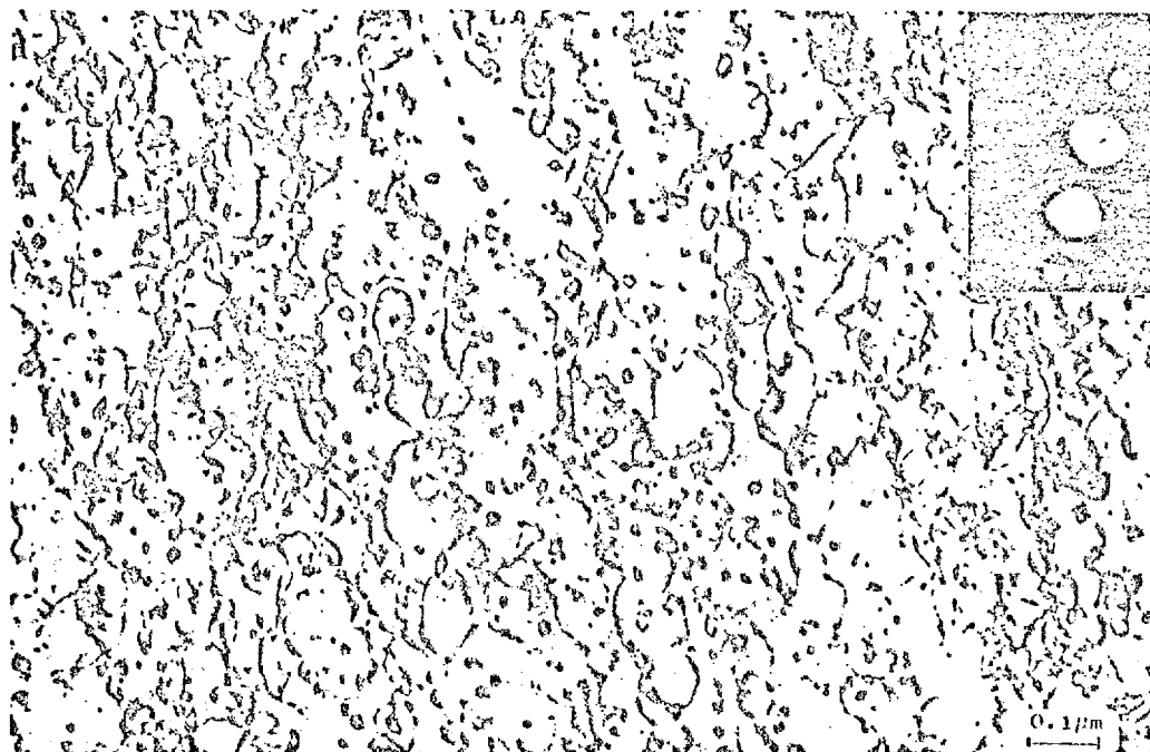
Fig. 9. Electron micrographs of the thin slice and electron diffraction diagrams of light-alloy test piece 11-I: (a) surface hardened zone; (b) unchanged part. Conditions of identical contrast in both cases.
