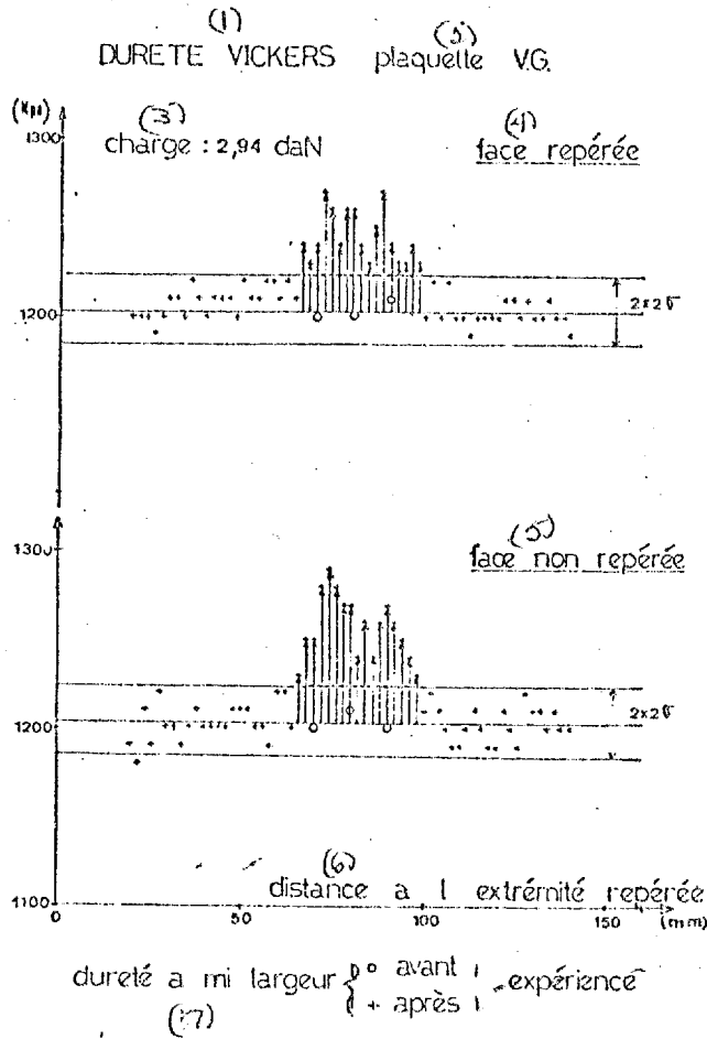
Fig. 8. Hardness measured on the two sides of light-alloy test piece VG, before and after test. KEY: (1) Vickers hardness. (2) Plate VG. (3) Load. (4) Marked side. (5) Unmarked side. (6) Distance to marked end. (7) Hardness at mid-width (°) before/ (+) after experiment.
