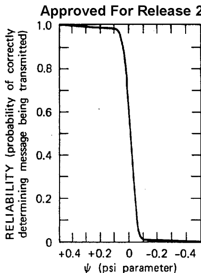
Fig. 19. Reliability curve for sequential sampling procedure ( p_0 = 0.4 , p_1 = 0.6 , \alpha = 0.01 , \beta = 0.01 ).
