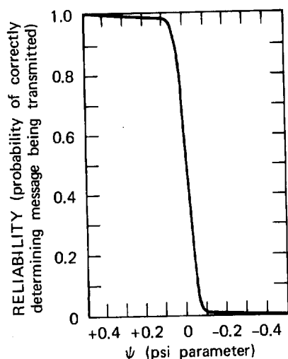
Fig. 19. Reliability curve for sequential sampling procedure ( p_0 = 0.4 , p_1 = 0.6 , \alpha = 0.01 , \beta = 0.01 ).
