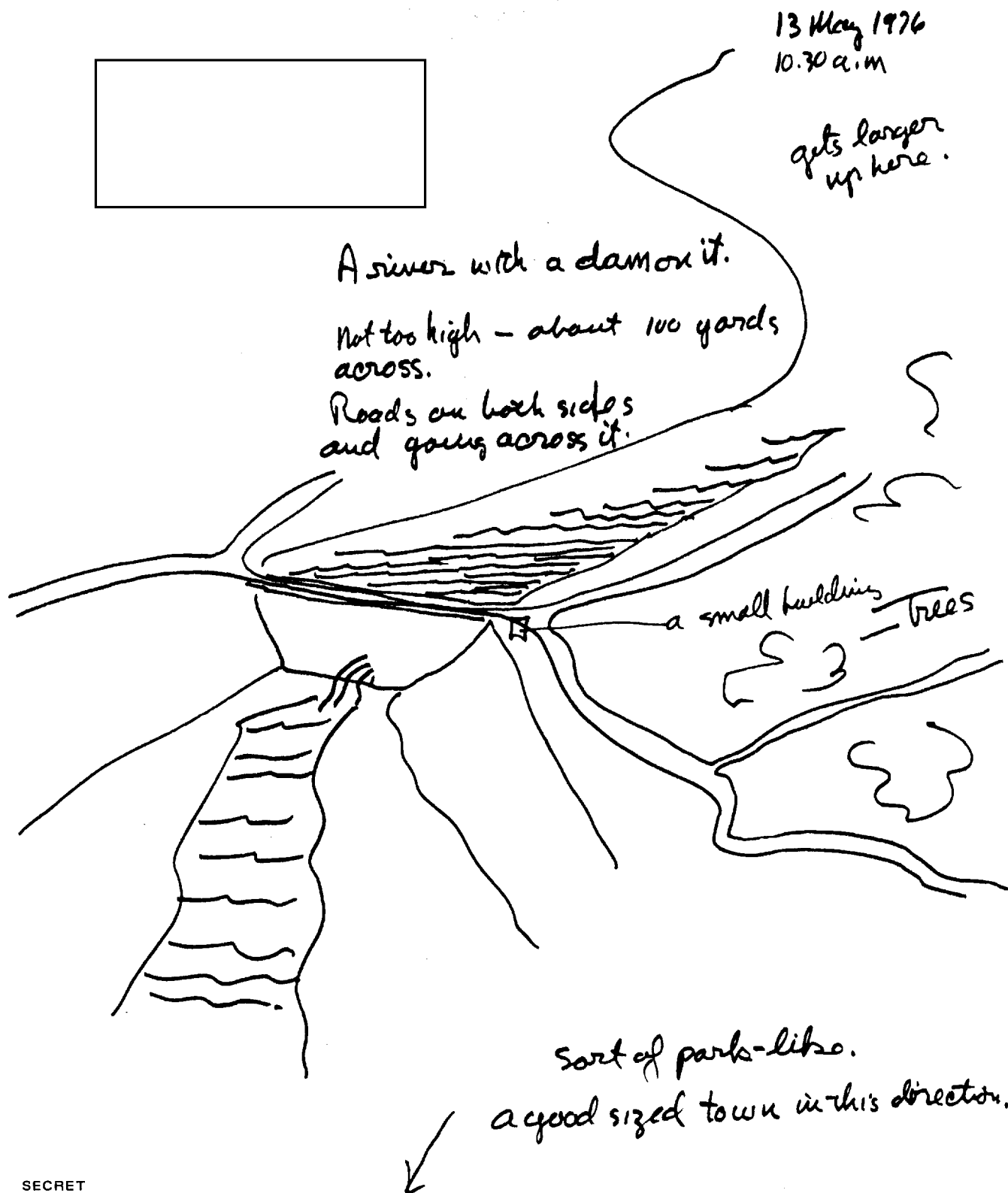
FIGURE B-5 REMOTE VIEWING BY GEOGRAPHICAL COORDINATES OF DAM SITE IN THE USSR (S)
