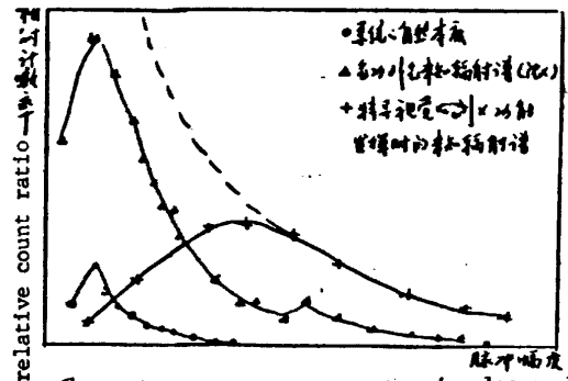
图8: 人体未知辐射的计数脉冲幅度谱 Fig. 8. Impulse amplitude spectrum of unknown human body radiation: ● - natural film, ▲ - unknown radiation produced by a person with trained ability (Shen), + - unknown radiation produced during exercise of "exceptional vision" ability.
