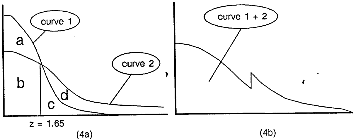
Figure 4. Method of estimating filedrawer size (see text)
