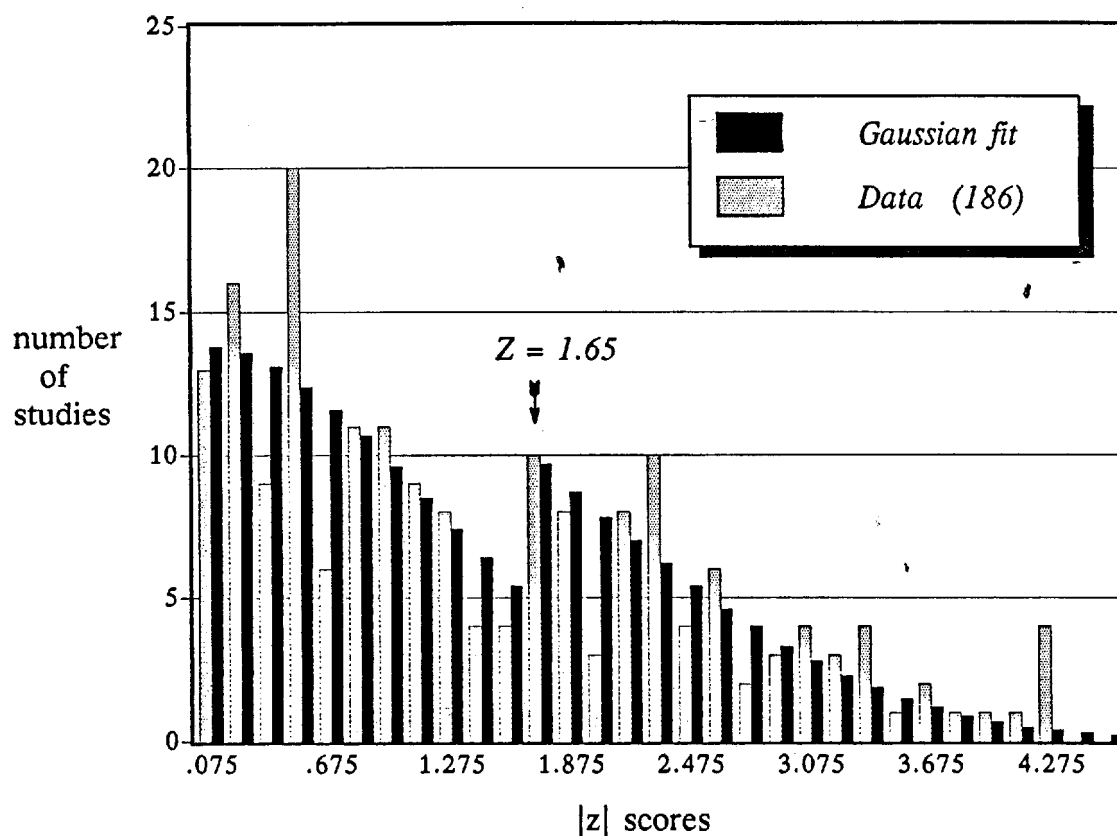
Figure 3. |z| score distribution for 186 survey experiments
