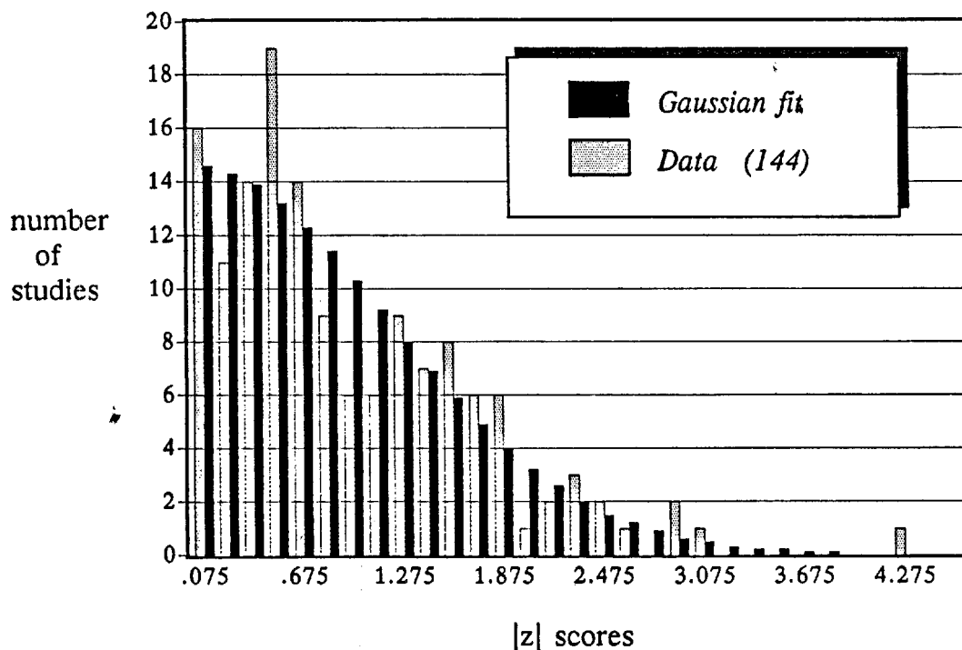
Figure 1. |z| score distribution for Princeton data
