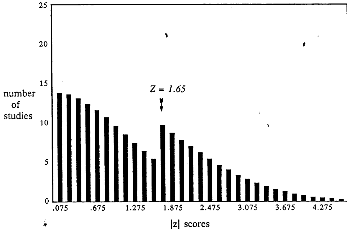
Figure 2. |z| score distribution with filedrawer problem
