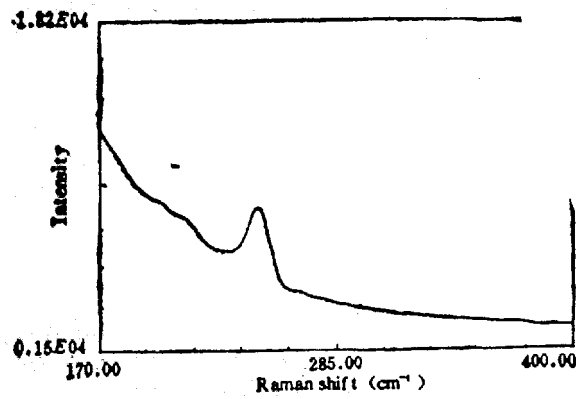
Fig. 2 Raman spectrum diagram of normal medical 0.9% physiological saline
