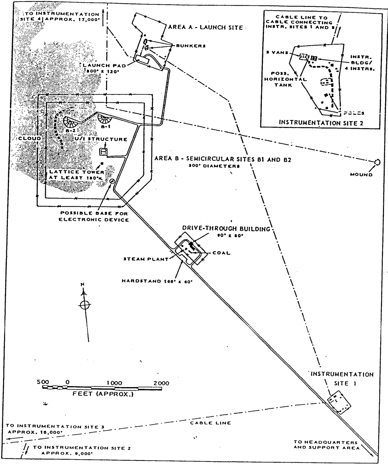
MISSILE LAUNCH COMPLEX B, SARY SHAGAN
