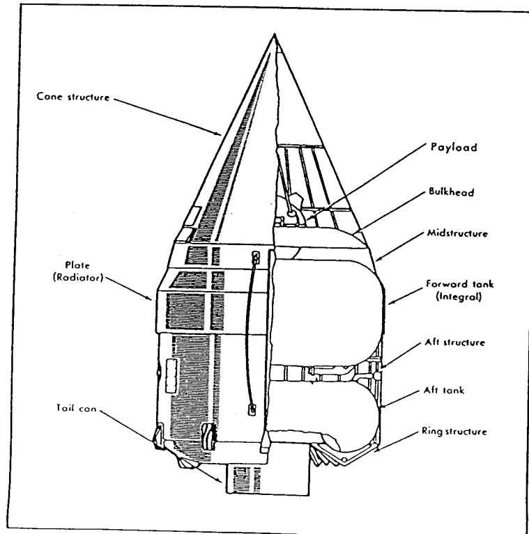
LUNIK UPPER STAGE
