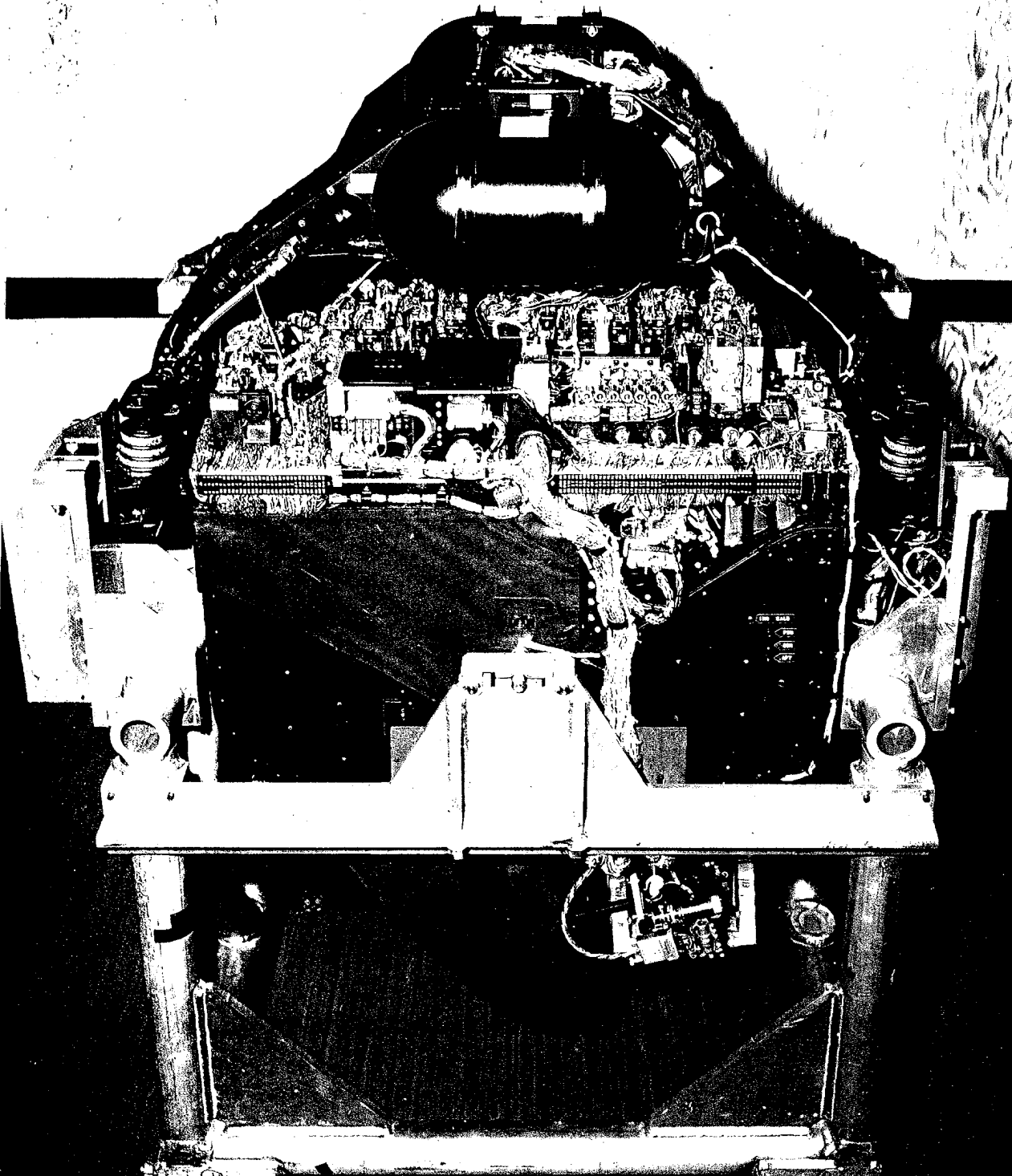
OXCART Perkin-Elmer Type I Camera carries 5000 feet of film on a single roll. It has a lens of 18 inches focal length and design objective of 1.2 feet ground resolution from an altitude of 85,000 - 90,000 feet.
