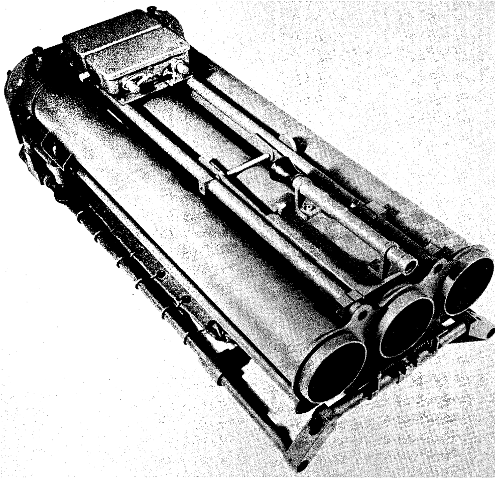
Figure 1 Launcher, Closed Position
