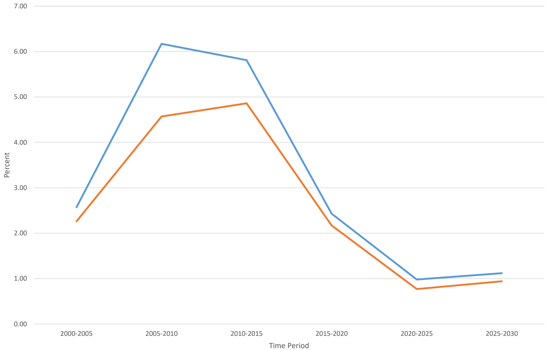
Jordan - Rate of Urbanization v. Rate of Total Population Growth
